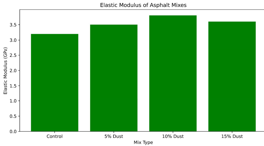
Fig. 2. Elastic Modulus Comparison Chart
