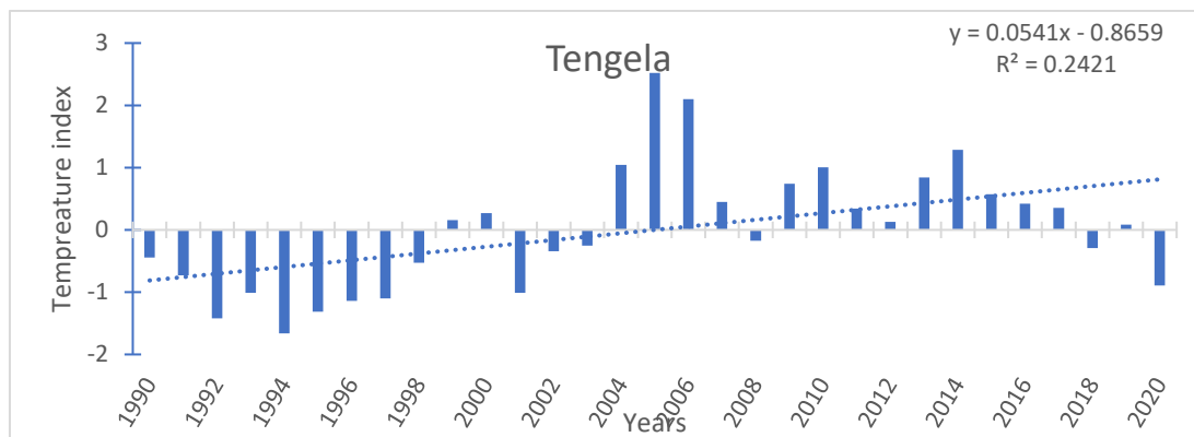
Fig. 3. Interannual temperature variability in Bagoué region from 1990 to 2020
