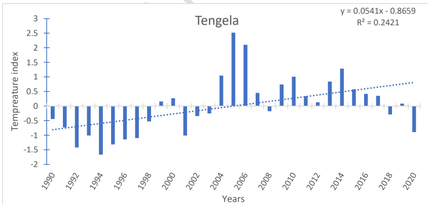
Fig. 3. Interannual temperature variability in Bagoué region from 1990 to 2020
