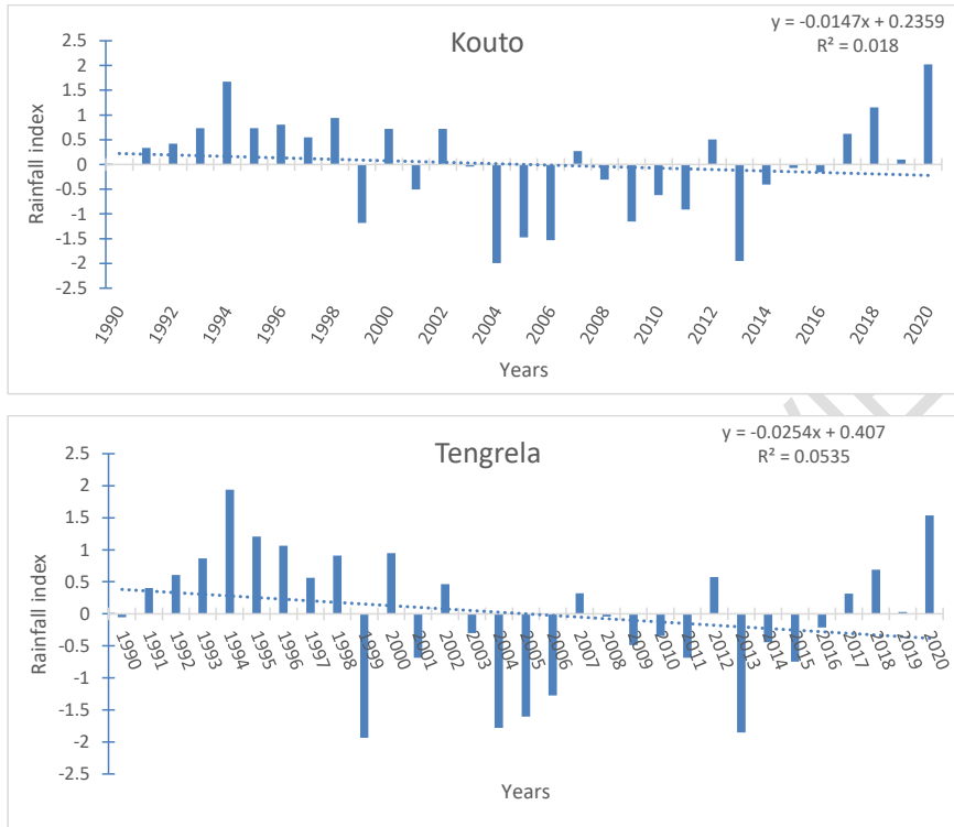
Fig. 2. Interannual rainfall variability in Bagoué region from 1990 to 2020.
