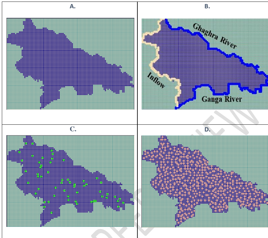
Fig 3. (A): Grid generated for modelling domain; (B): Map showing boundary conditions in the study area; (C): The location of observation wells in the model area; (D): The distribution of pumping well in the study area
