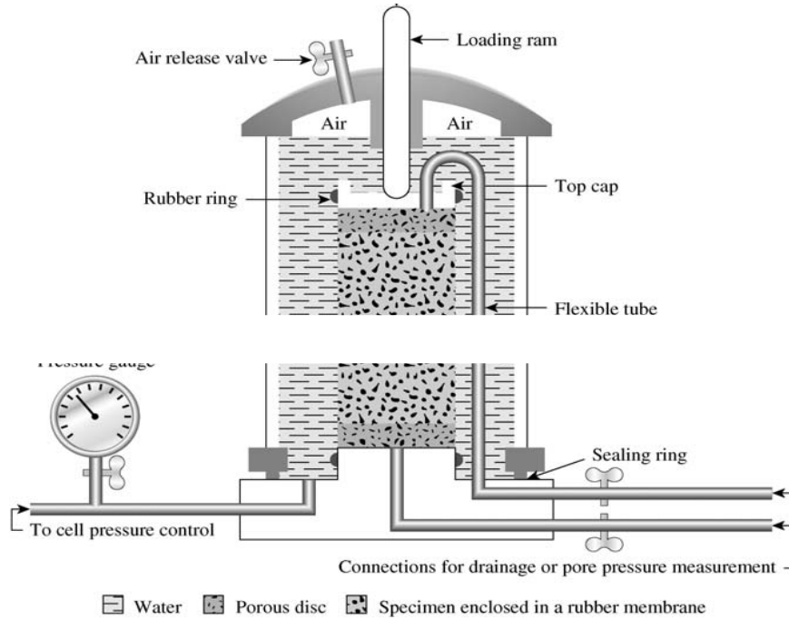
Figure 1: A Diagram of the Triaxial Test Equipment.
