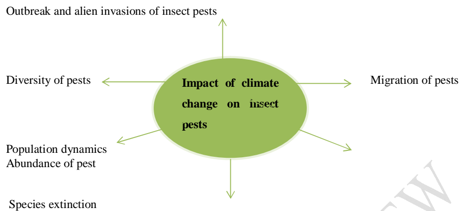
Fig. 1 Impact of climate change on insect pests
