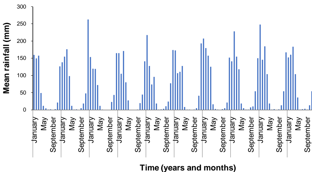
Figure 2: Monthly rainfall of the Usangu catchment
