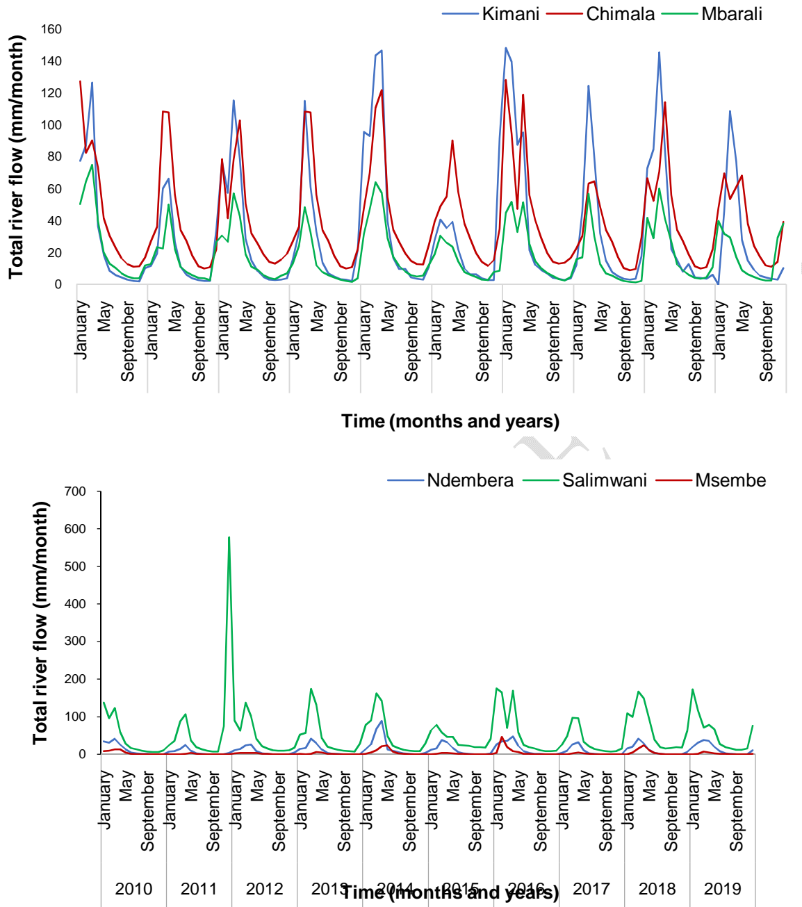
Figure 3: Monthly specific discharge data for the six rivers
