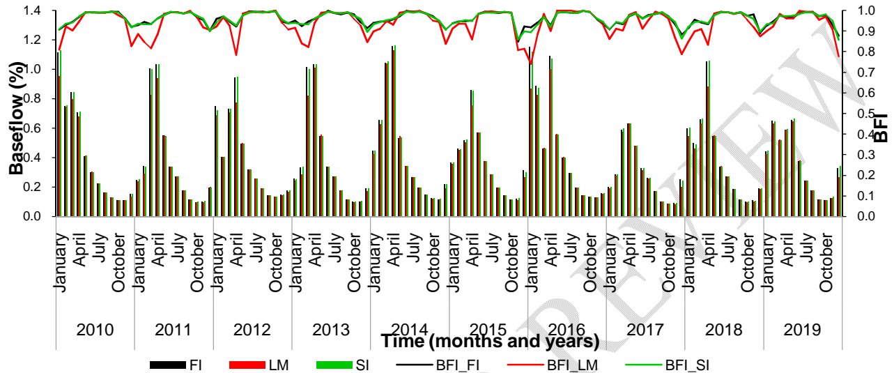
Figure 5: Baseflow separation techniques along with BFI for Chimala at Chitekelo
