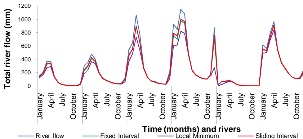
Figure 4: Comparison of baseflow separation methods against total river flow
