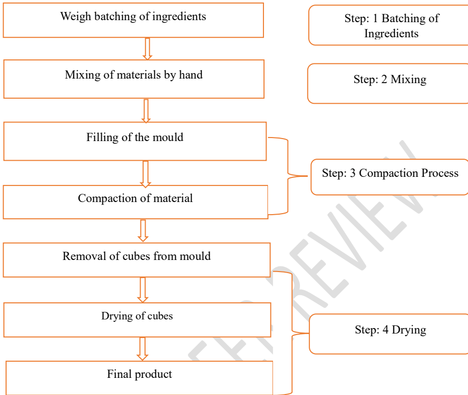
Figure 3 Flow chart of the manufacturing process of concrete based on hemp shiv
