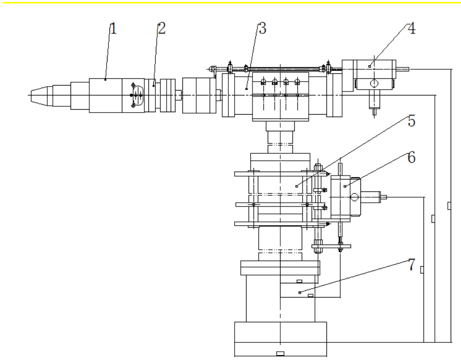
Fig.1 Main view of welding manipulator shape
