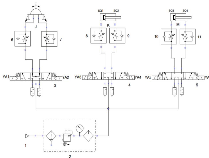
Fig.7 Mechanical arm pneumatic drive system circuit
