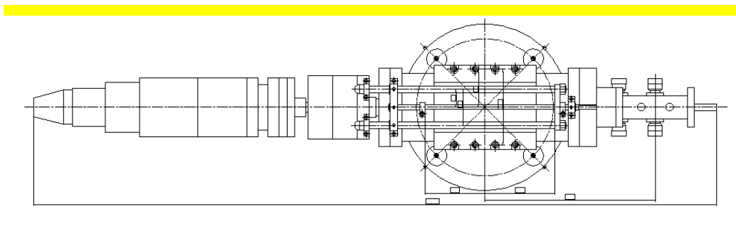
Fig.2 Top view of welding manipulator shape
