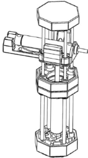
Fig. 6 Lifting structure of large arm of manipulator
