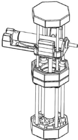
Fig. 6 Lifting structure of large arm of manipulator
