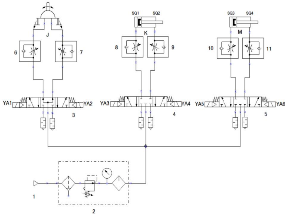
Fig.7 Mechanical arm pneumatic drive system circuit
