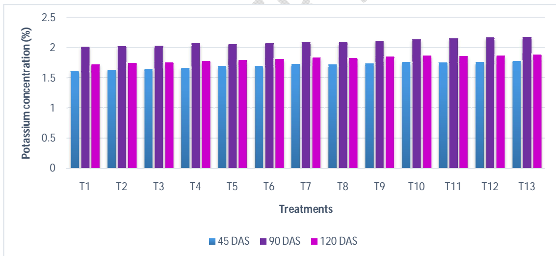
Figure 8. Influence of zinc and silica solubilizing bacterial isolates and their consortia on potassium concentration (%) of plant in pot culture experiment
