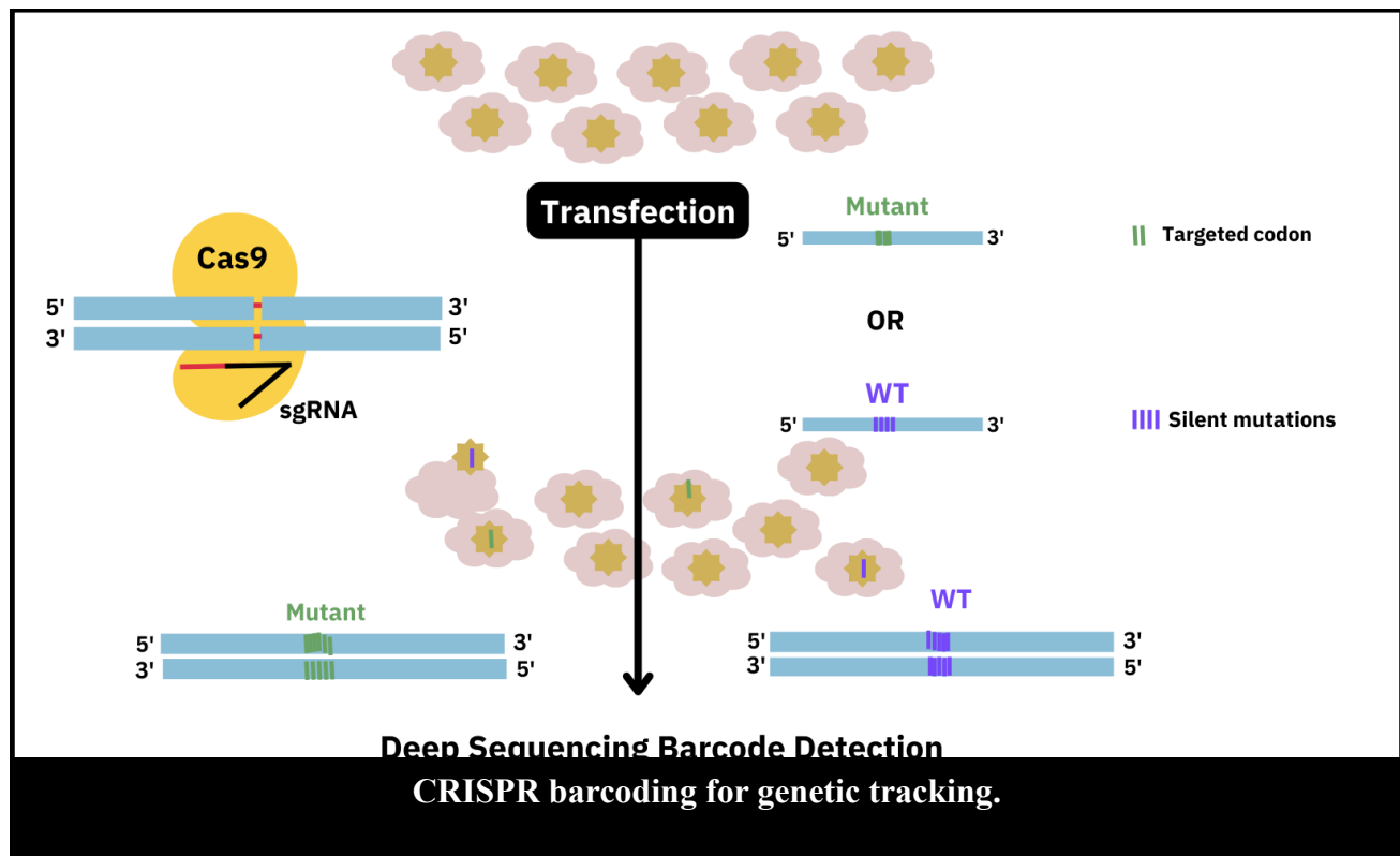
fig. 4 CRISPR barcoding for genetic tracking.
