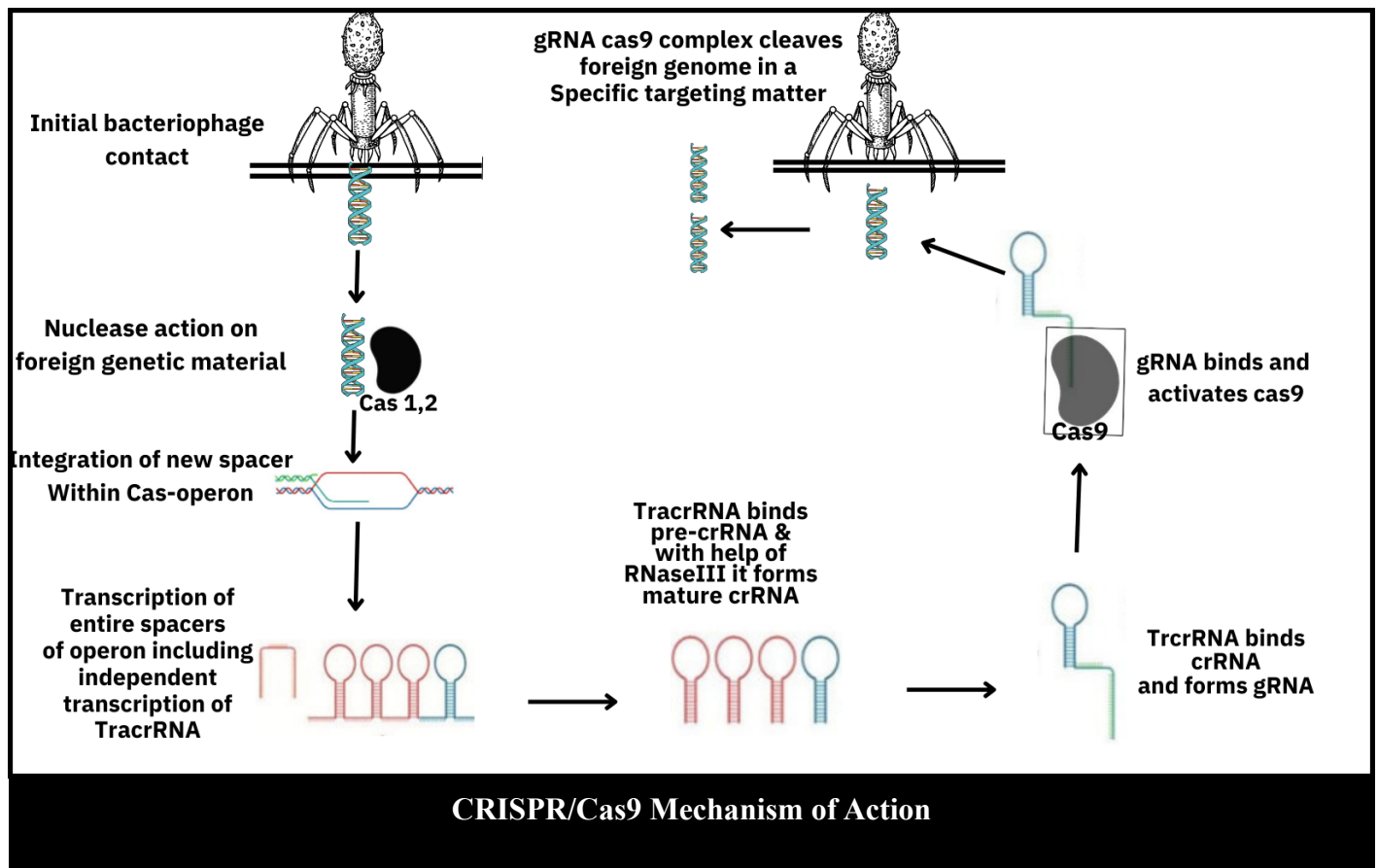
fig. 1 CRISPR/Cas9 Mechanism of Action
