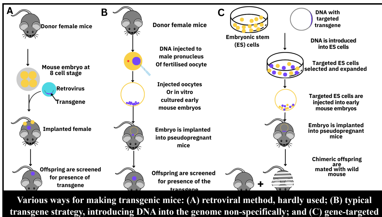
fig.3 Various ways for making transgenic mice: (A) retroviral method, hardly used; (B) typical transgene strategy, introducing DNA into the genome non-specifically; and (C) gene-targeted
