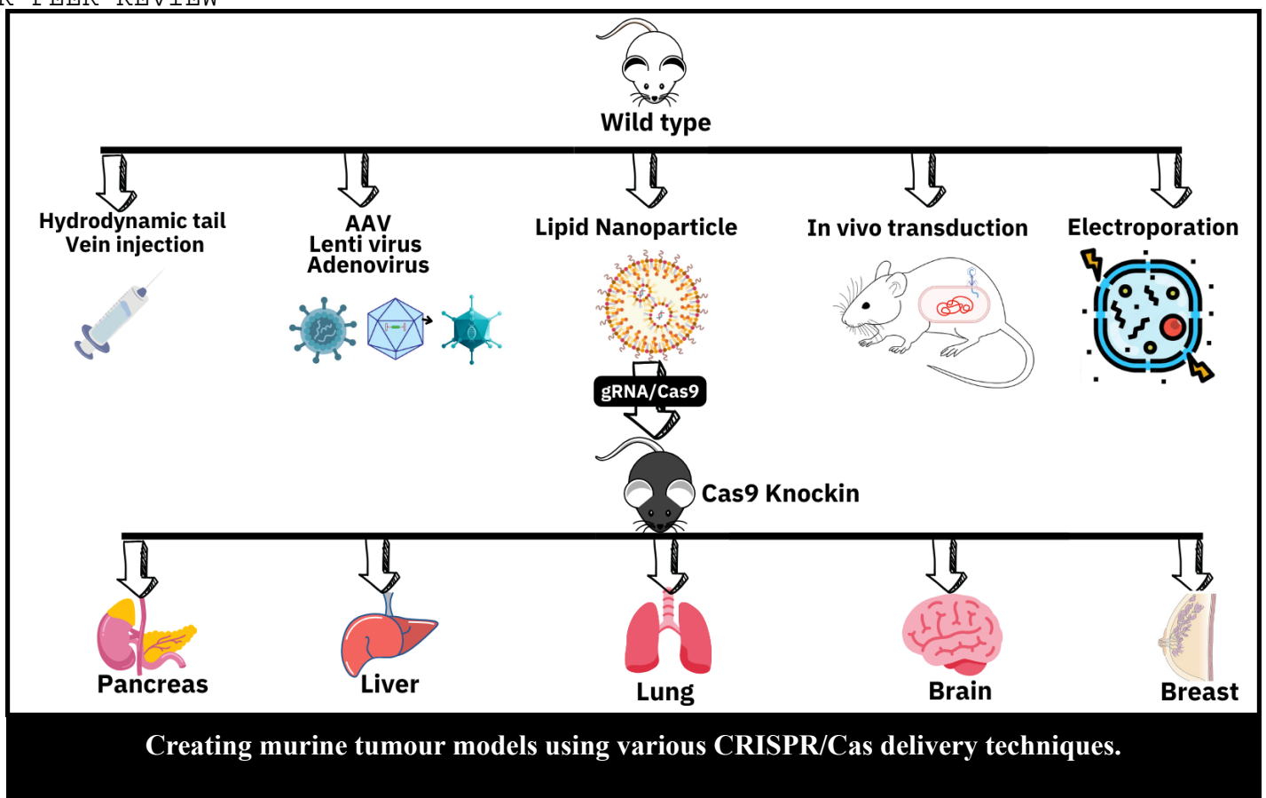
fig.2 Creating murine tumour models using various CRISPR/Cas delivery techniques.
