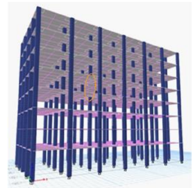
Fig. 3 Details of the Model with Static column removal for Regular Framed Building
