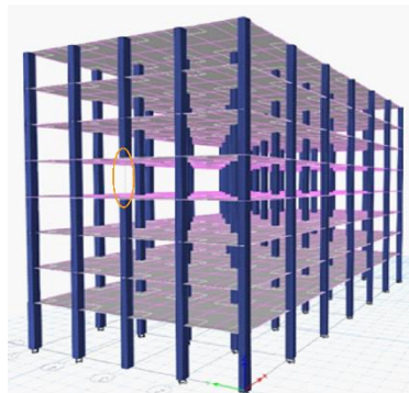
Fig. 3 Details of the Model with Static column removal for Regular Framed Building
