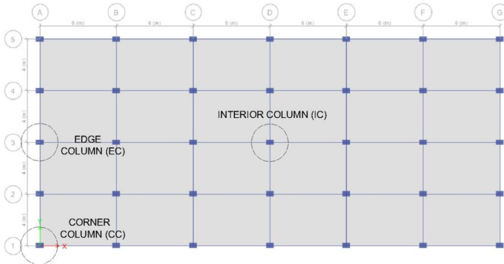
Fig. 1 Plan of the 8-storey Building
