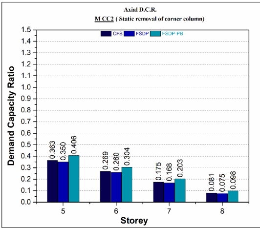
Fig. 10 DCR for axial forces of column MCC2 on the removal of middle floor corner column (a) static removal (b) dynamic removal
