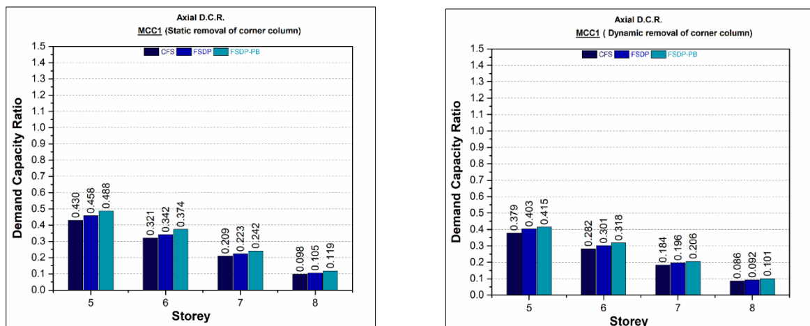
Fig. 8 DCR for axial forces of column MCC1 on the removal of middle floor corner column (a) static removal (b) dynamic removal
