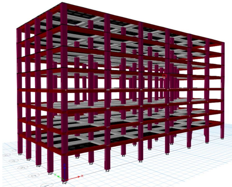
Fig. 2 Three dimensional geometry of the 8-storey Building
