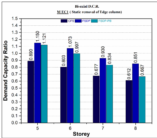
Fig 13 DCR for biaxial forces of column MEC1 on the removal of middle floor edge column (a) static removal (b) dynamic removal
