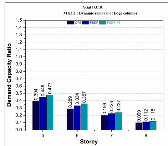
Fig. 14 DCR for axial forces of column MEC2 on the removal of middle floor edge column (a) static removal (b) dynamic removal
