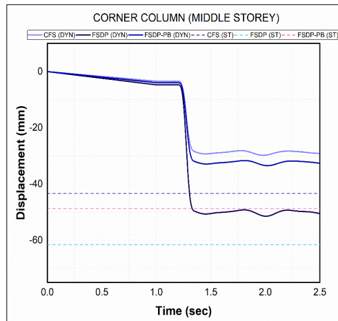
Fig. 20 Time history response of vertical displacement when CC is instantaneously removed at t = 1.25 s for buildings CFS, FSDP, and FSDP-PB along with static displacement response on intermediate storey
