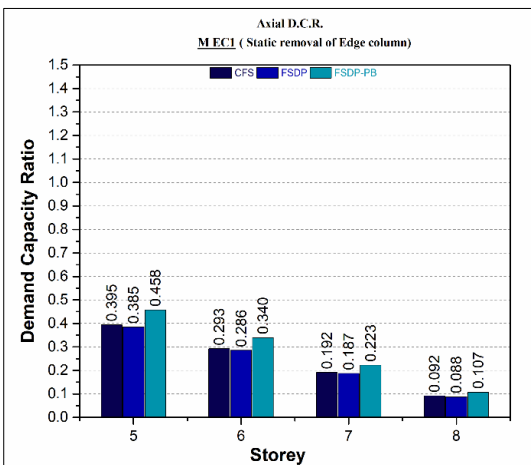
Fig 12 DCR for axial forces of column MEC1 on the removal of middle floor edge column (a) static removal (b) dynamic removal
