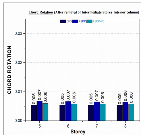
Fig. 25 Chord Rotation when Interior column is statically removed for buildings CFS, FSDP, and FSDP-PB on intermediate storey
