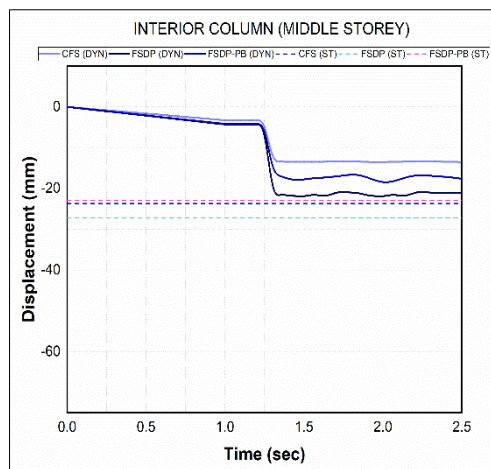
Fig. 22 Time history response of vertical displacement when IC is instantaneously removed at t = 1.25 s for buildings CFS, FSDP, and FSDP-PB along with static displacement response on intermediate storey
