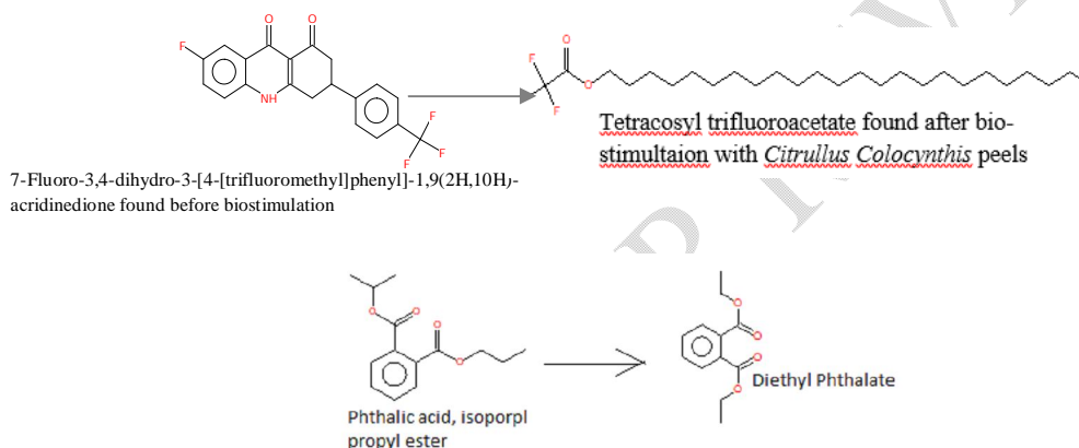
Fig 11 :Chemical transformation
