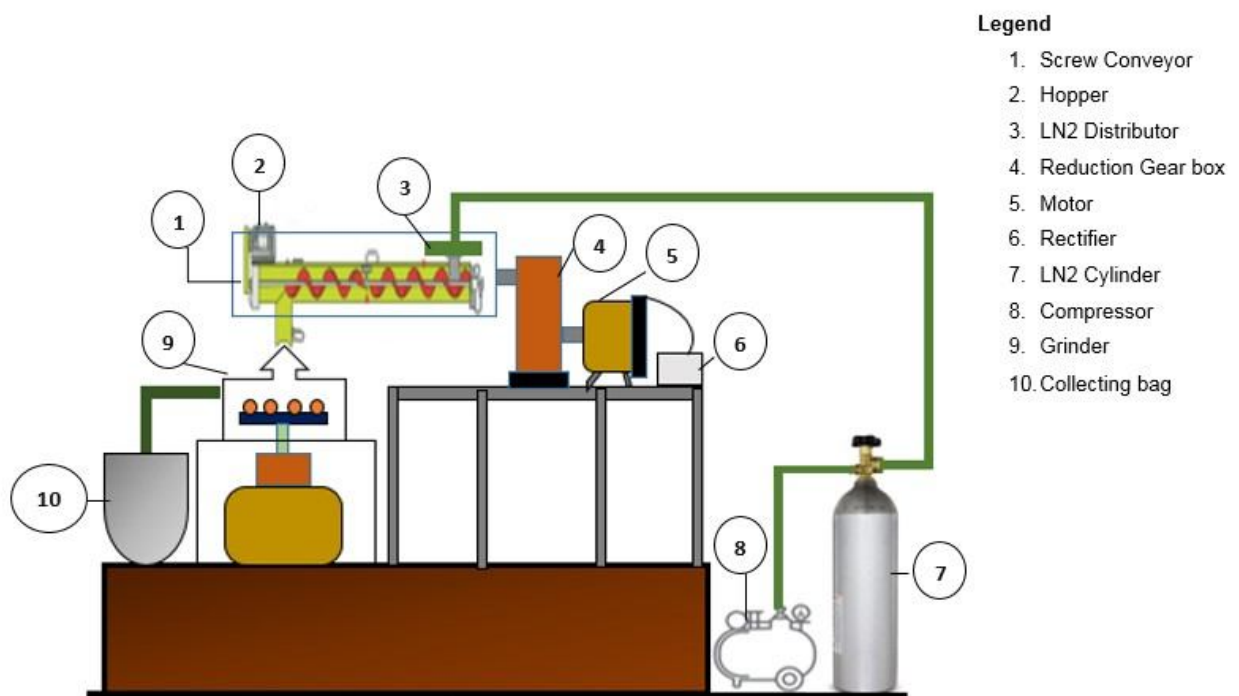
Figure 1. Cryomilling system
