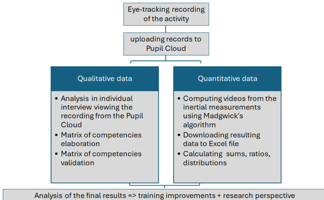
Fig. 2. Overview of the method: the chart flow illustrates the qualitative and quantitative processing of the data
