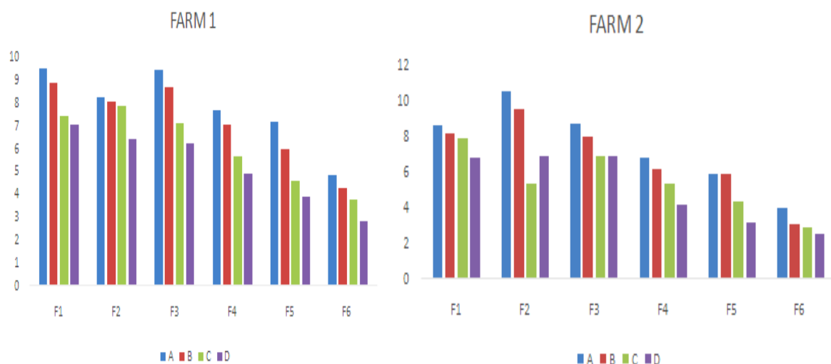
Fig 7: Concentration of iron. A = 3 mm-deep dry sediment [flooded area]; B = 30 cm deep; not including dry sediment [flooded area] C = 3 mm-deep surface soil [non-flooded area]; D = 30 cm deep; not including surface soil [non-flooded area]. Y-axis = concentration of metal in mg/kg.
