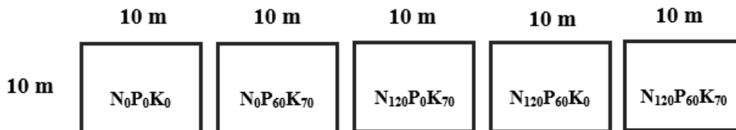
Figure 1 : Experimental setup
