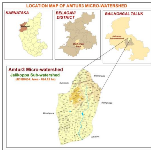
Fig.1. Location map of Amtur-3 micro-watershed
