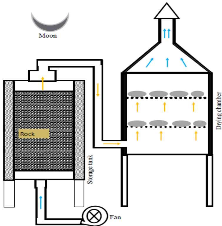
Figure 2: Dryer operation after sunset
