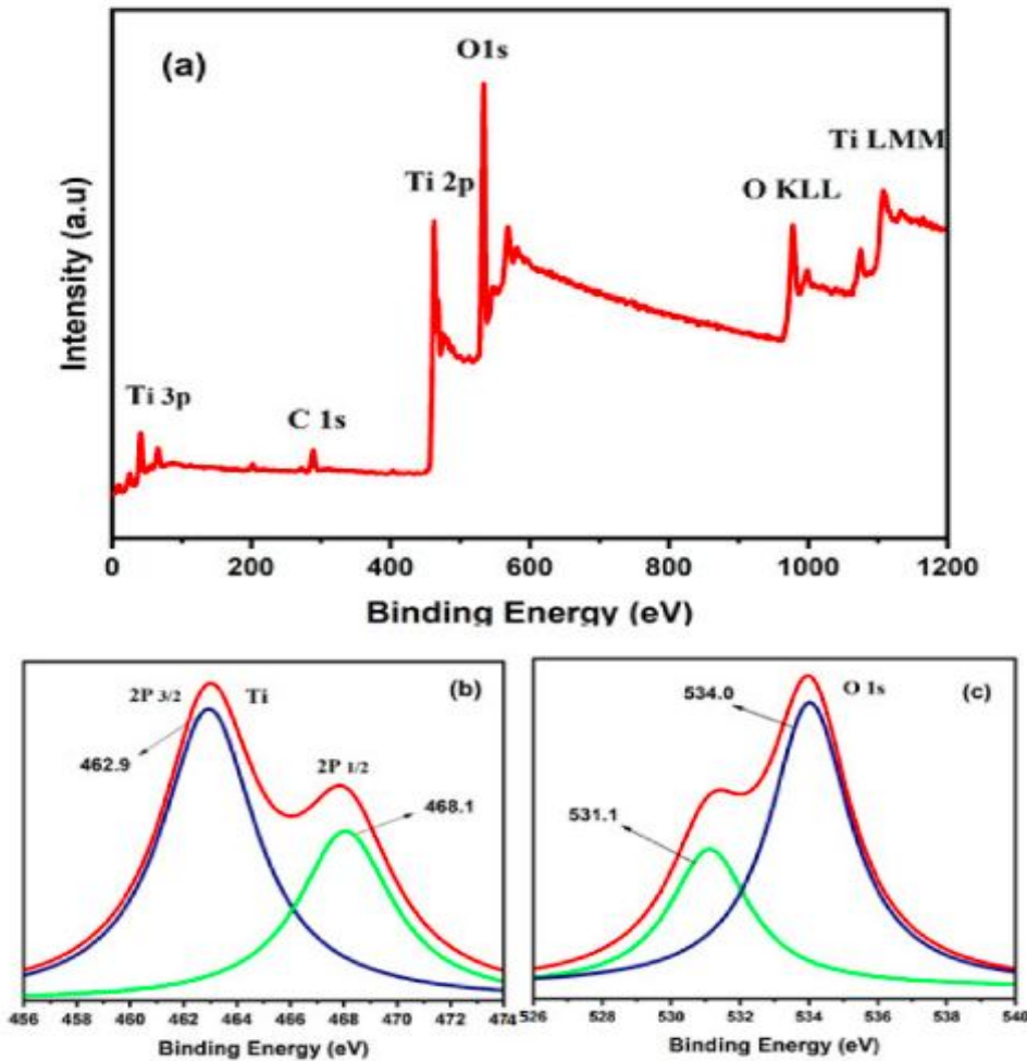
Fig. 9. XPS analysis of Titanium dioxide nanoparticles [66].
