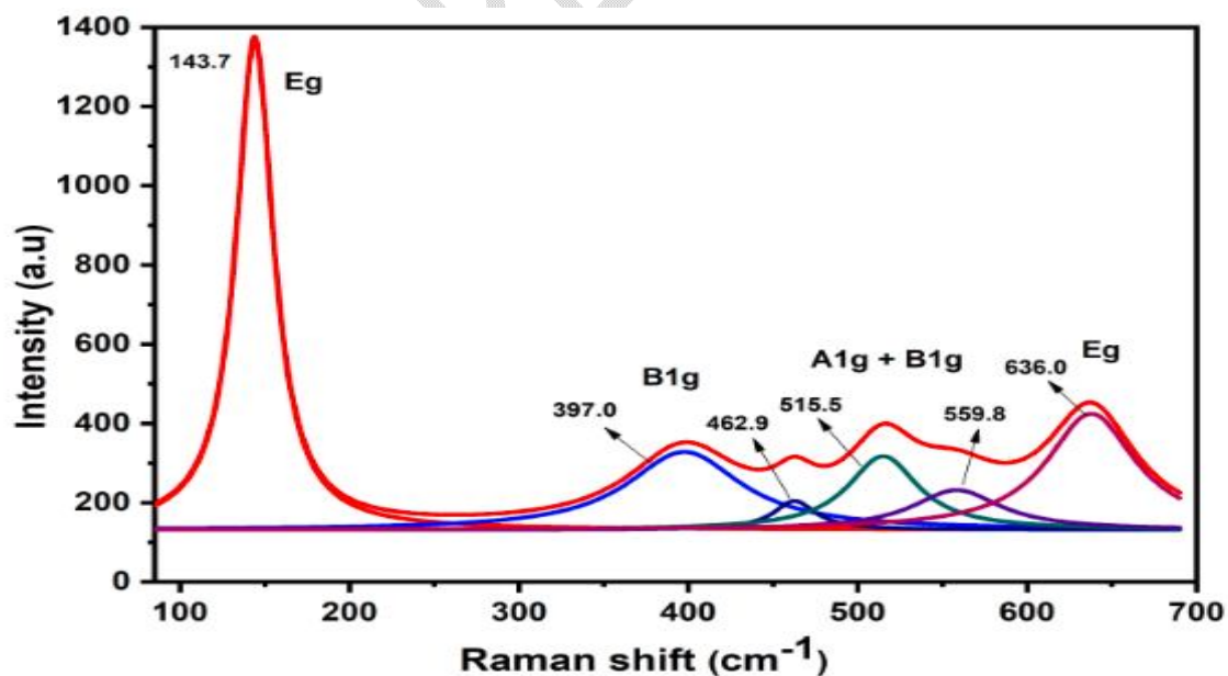
Fig. 13. Raman spectrum of Titanium dioxide nanoparticles [66].
