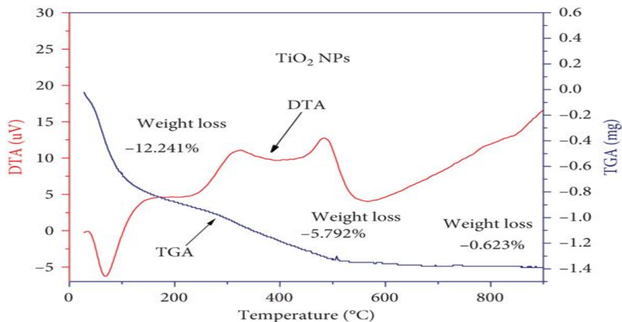
Fig. 12. TGA/DSC analysis of \text{TiO}_2 nanoparticles [72].
