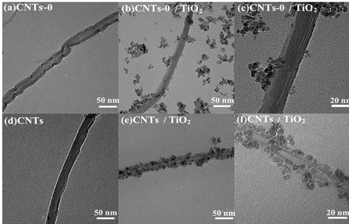
Fig. 6. TEM image of Titanium dioxide particles and carbon nanotubes. Reprinted with permission ref[63]. Copyright 2020, Elsevier.
