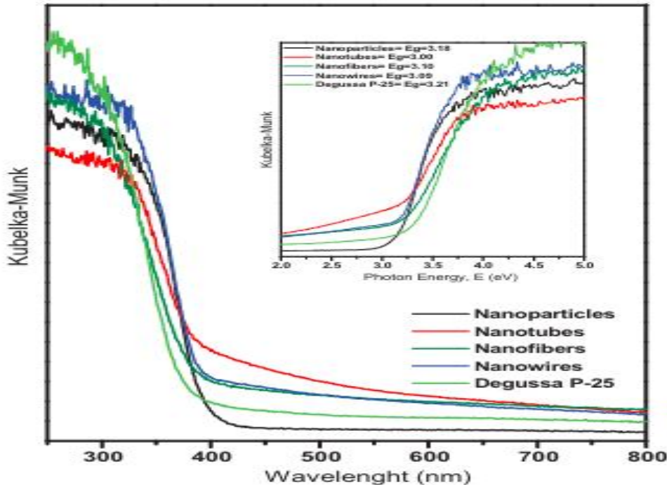
Fig. 14. UV-Vis spectrum of nanoparticles, nanotubes, nanofibers, nanowires, and P-25. Reprinted with permission ref[78]. Copyright 2016, Elsevier.
