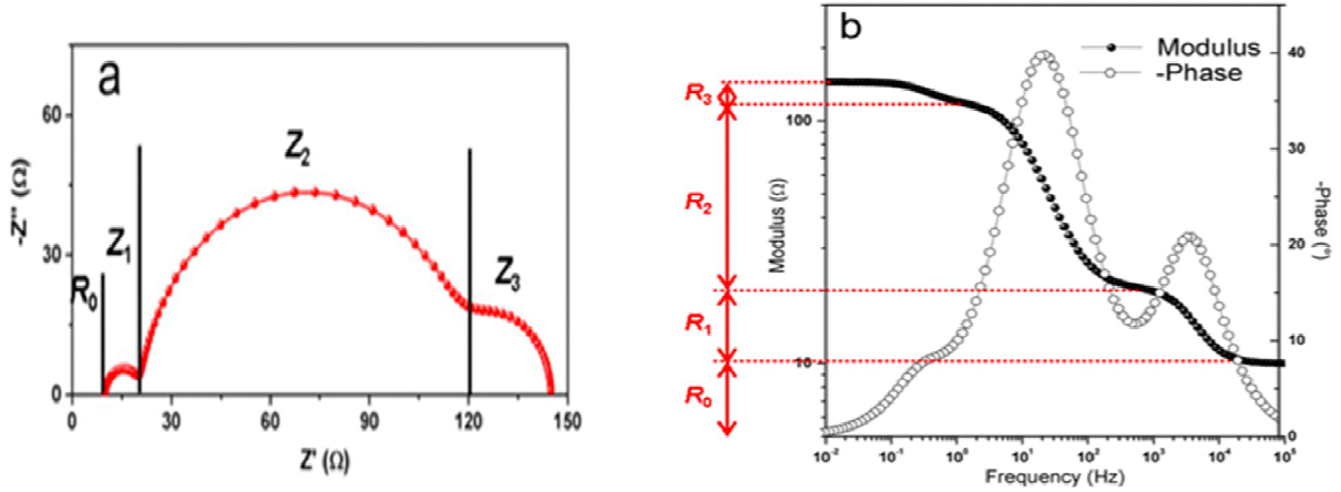
Fig. 4. A schematic representation of Nyquist (a) and Bode (b) Plots. Reprinted with permission ref[40]. Copyright 2017, Elsevier
