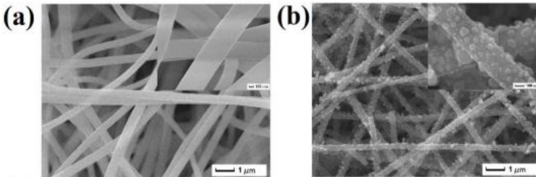
Fig. 5. SEM image (a) carbon nanofibers and (b) TiO 2 nanoparticles-carbon nanofibers.Reprinted with permission ref[62]. Copyright 2019, Elsevier.
