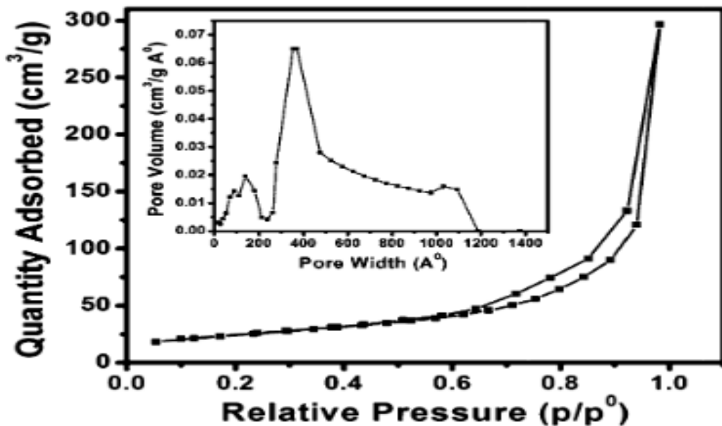
Fig. 11. Nitrogen desorption-adsorption isotherm of TiO 2 showing the pore volume insert [71].
