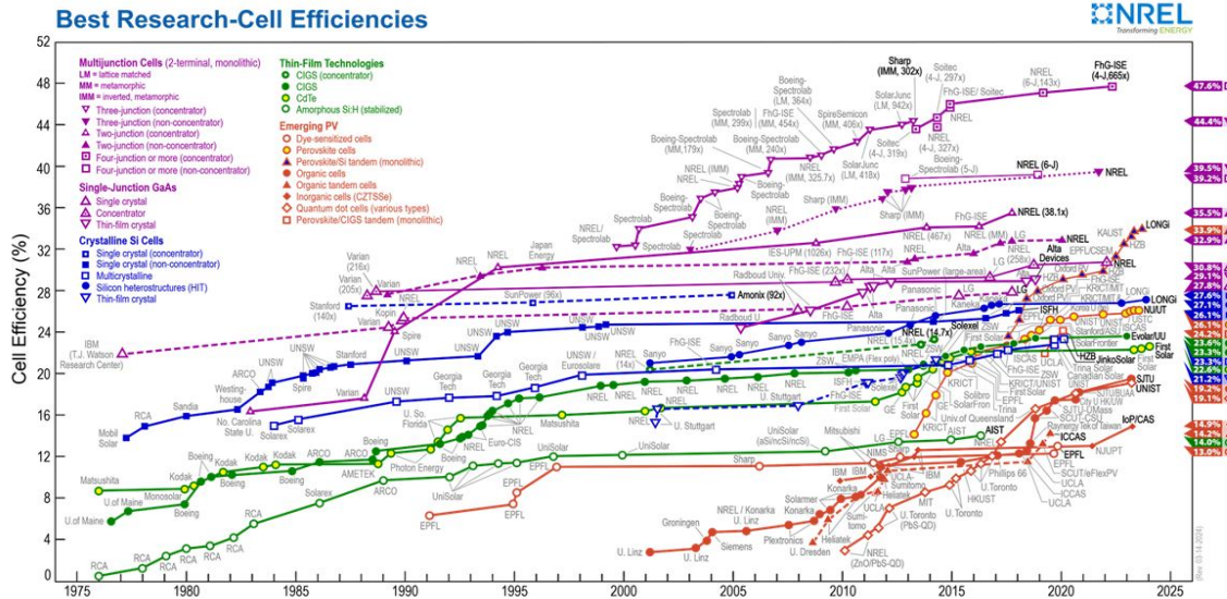
Fig. 1. Various solar-electricity conversion technologies over a range of 1975-2025.
