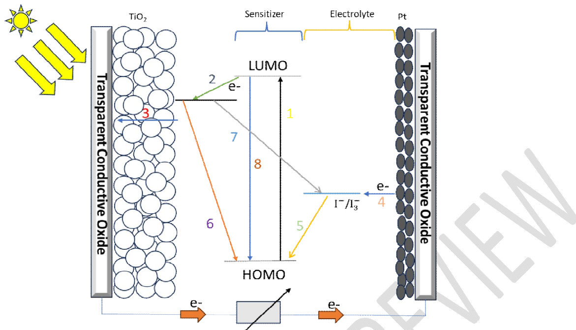
Fig. 2. Electron transfer in the various dye-sensitized solar cell components.
