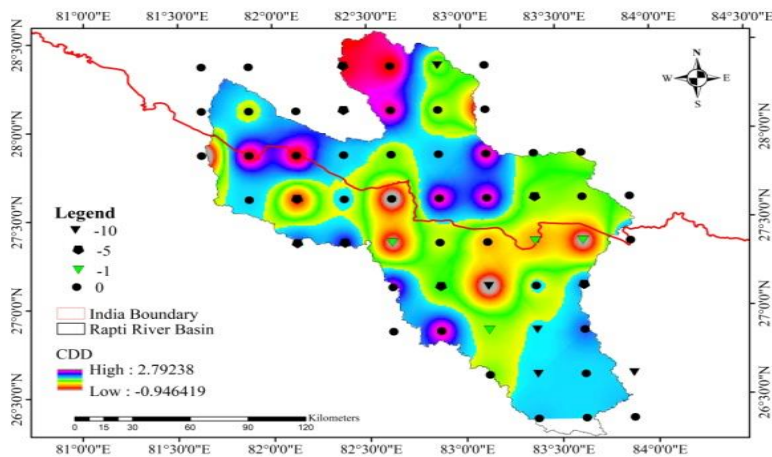
Figure 7: Trends of Consecutive Dry Days (CDD) at ACCESS-CM2 Model for 3°
