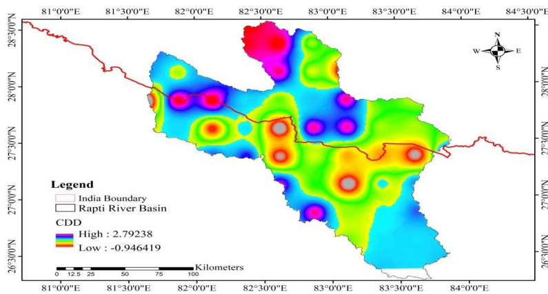
Figure 4: Consecutive Dry Days (CDD) at ACCESS-CM2 Model for 3°
