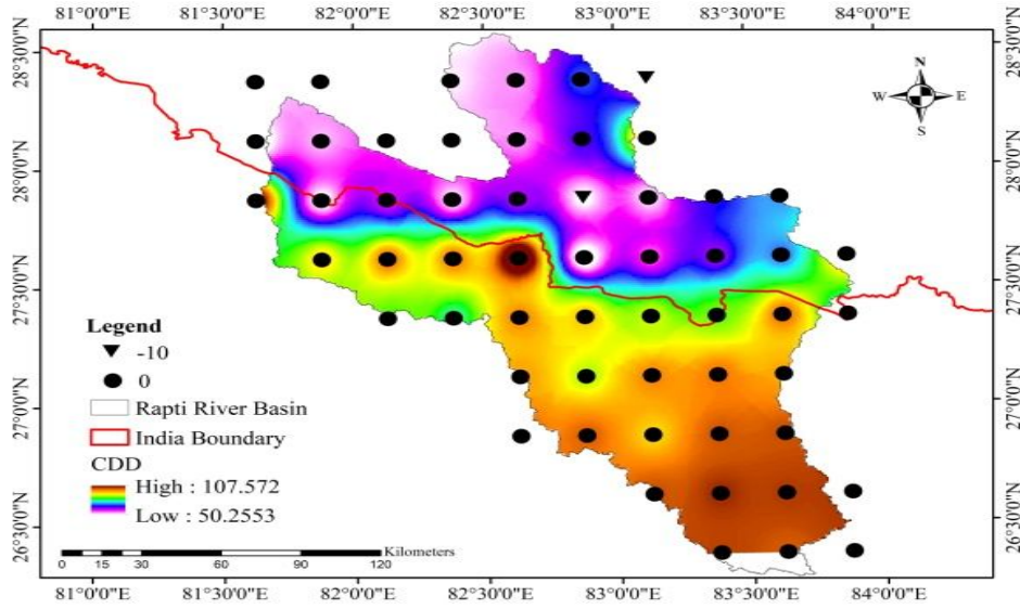
Figure 5: Trends of Consecutive Dry Days (CDD) at ACCESS-CM2 Model for 1.5°
