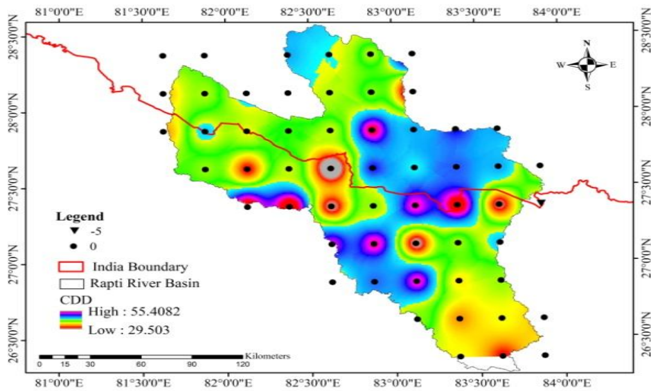
Figure 6: Trends of Consecutive Dry Days (CDD) at ACCESS-CM2 Model for 2°
