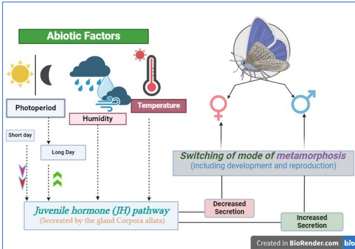
Figure 1 Abiotic factors causing sex ratio distortion in insects (61, Created with BioRender.com)
