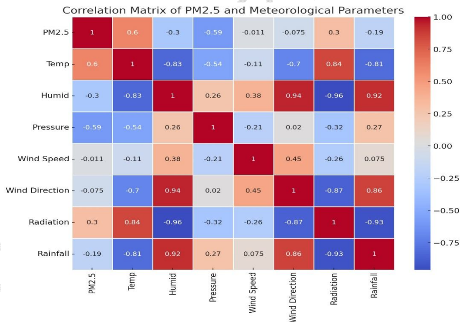
Fig. 1. Correlation between \text{PM}_{2.5} and the Meteorological Parameters
