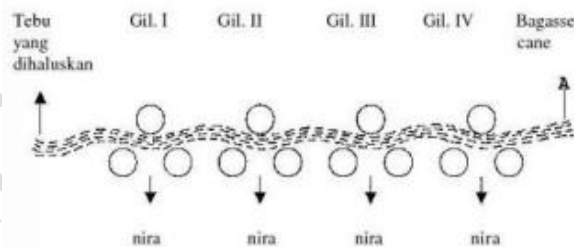
Figure 8. Sugarcane Milling Process (Source: [20])
