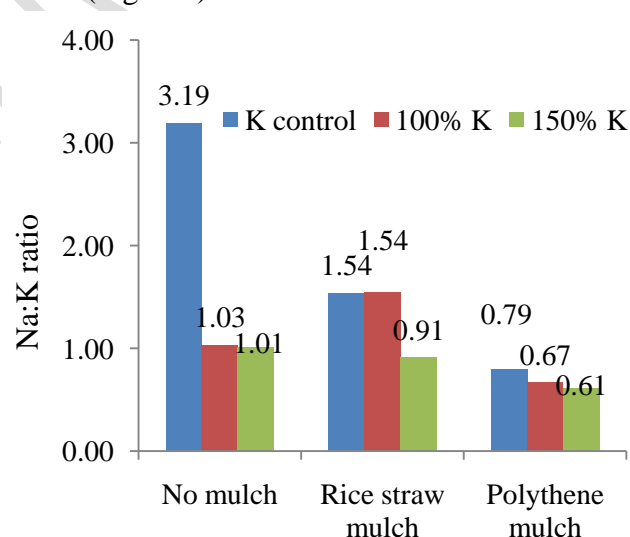
Fig. 3 Na:K ratio of bitter gourd leaf at Barguna district in the year 2018-19
