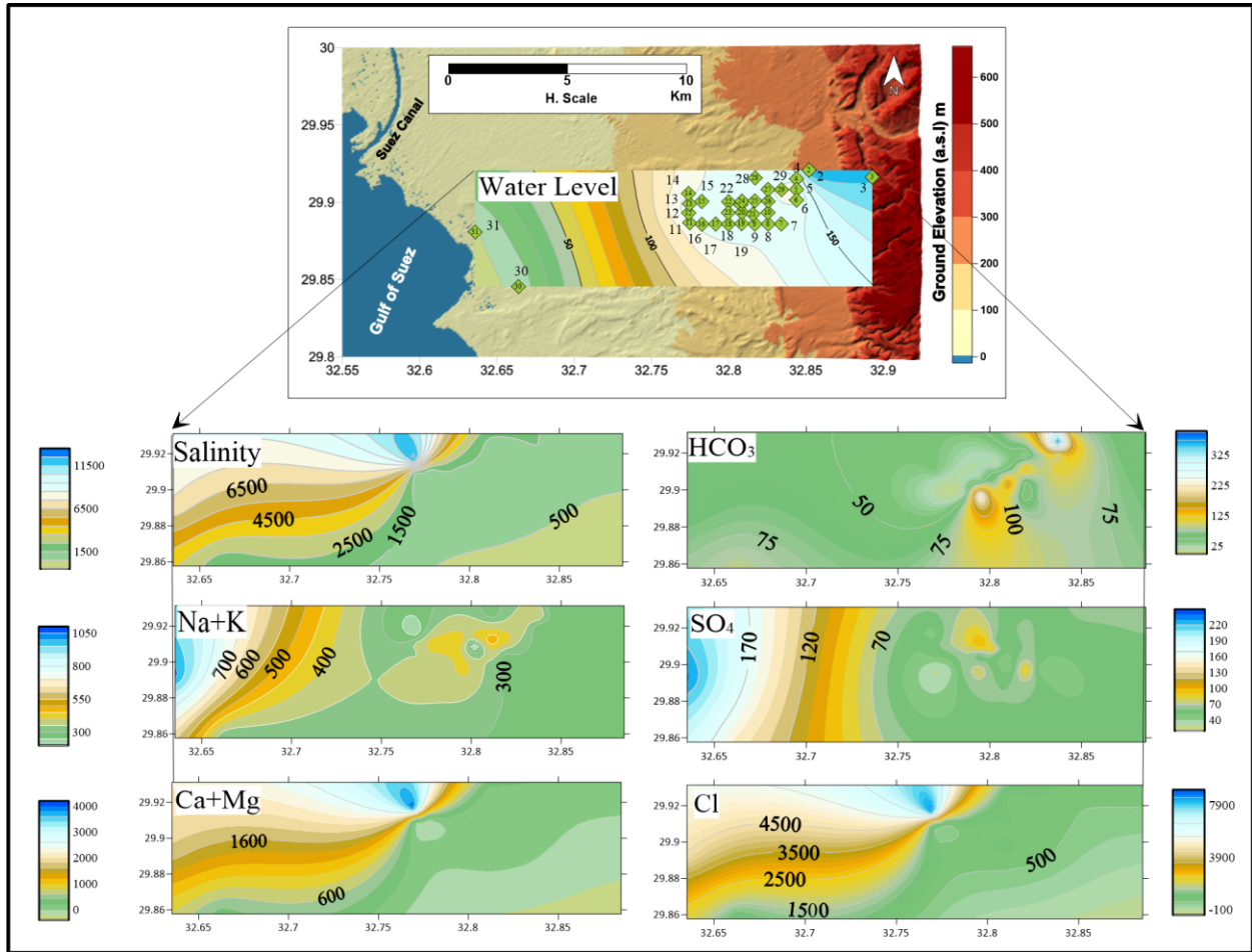
Figure 5. Spatial distribution of salinity, major cations (Na + K, and Ca + Mg in mg/L), and major anions (HCO 3 , SO 4 , and Cl in mg/L) in the groundwater of the Upper Cretaceous Aquifer, El Rina–Nihayaat, South Sinai, Egypt.
