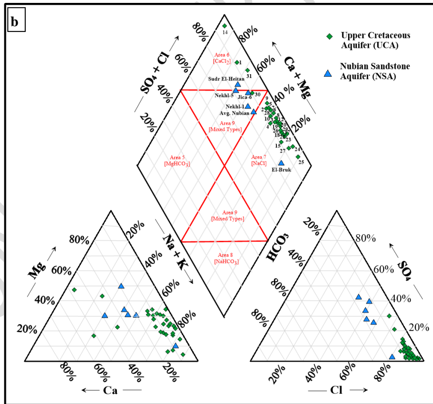
Figure 6.a) Gibbs diagram [45], and b) Piper Diagram [46], for groundwater samples tapping the Lower and Upper Cretaceous aquifer (UCA) in the Sinai Peninsula.
