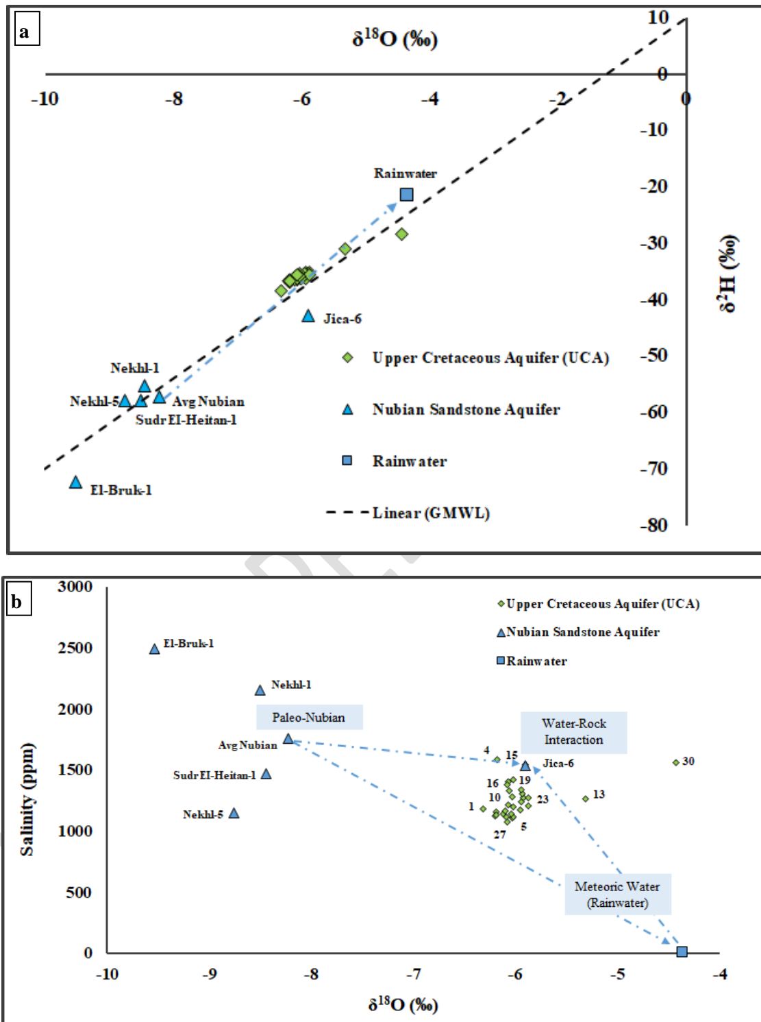
Figure 8. Relationships between \delta^{18}\text{O} (‰) versus; a) Deuterium ( \delta^2\text{H} ) (‰) and b) Salinity (mg/L) for groundwater samples tapping the Lower and Upper Cretaceous aquifer (UCA) in the study area.
