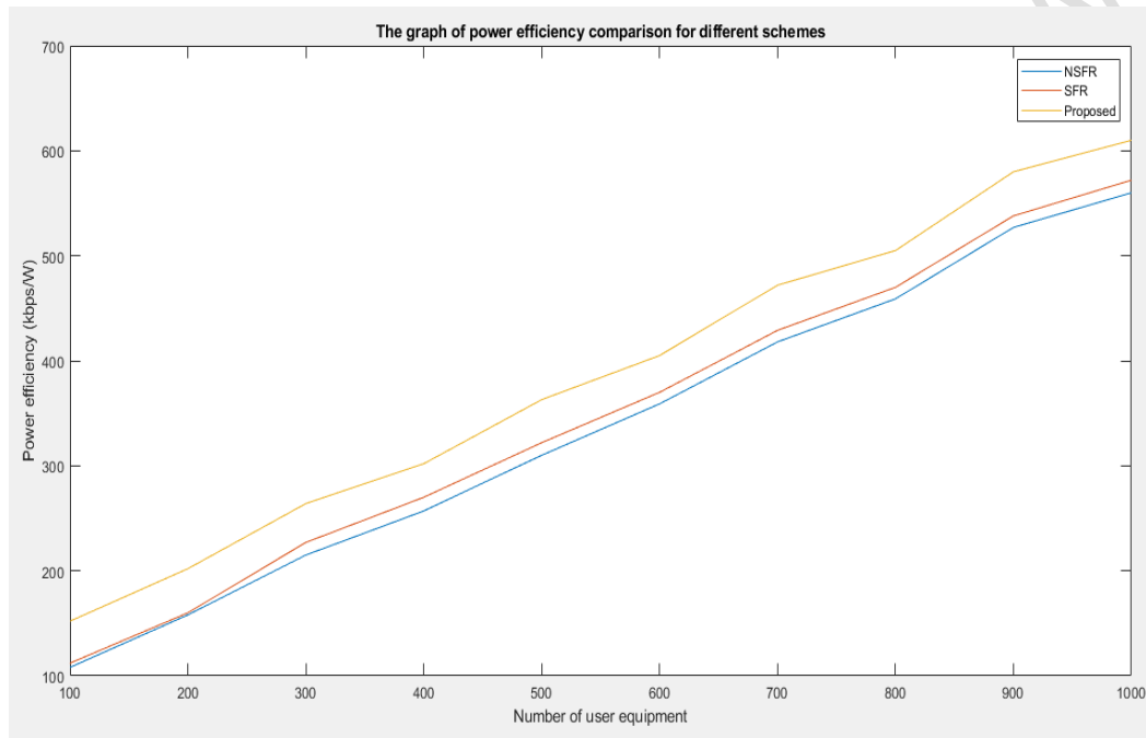
Figure 11. Power efficiency comparison of various schemes
