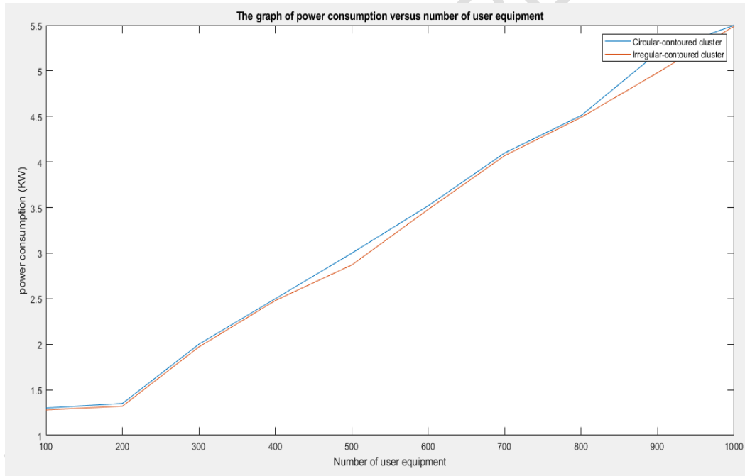
Figure 6. Power consumption versus the number of user equipment for circular-contoured cluster and irregular-contoured cluster
