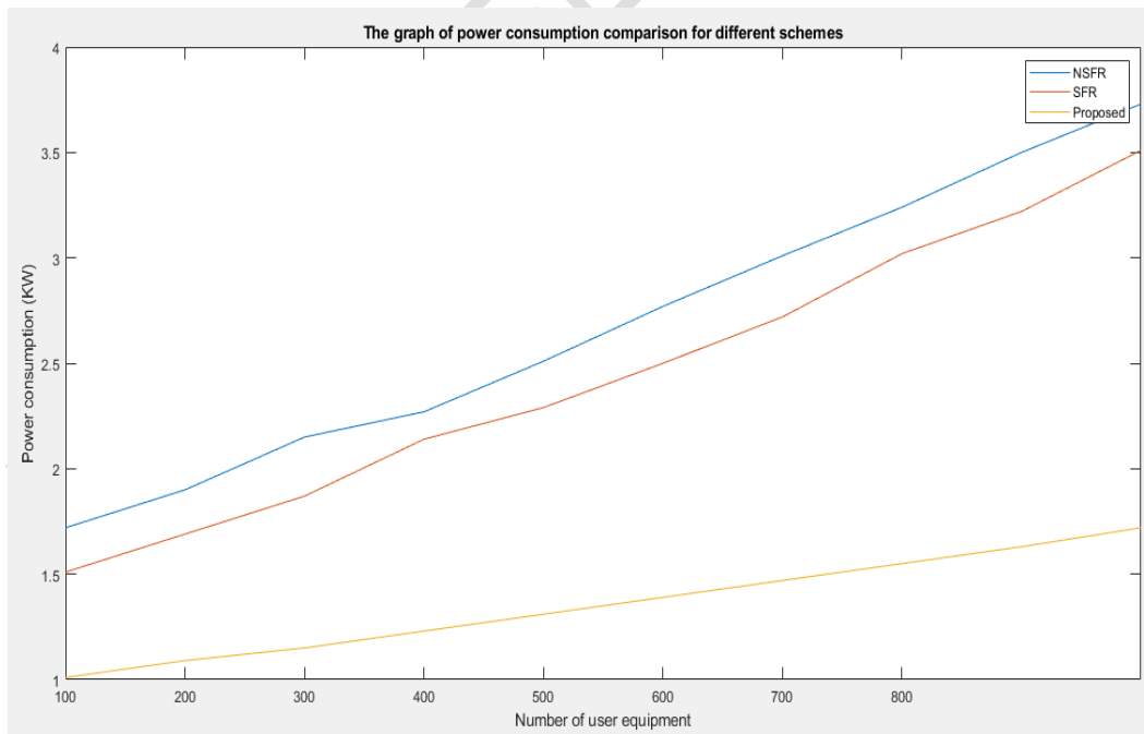
Figure 9. Power consumption versus the number of user equipment
