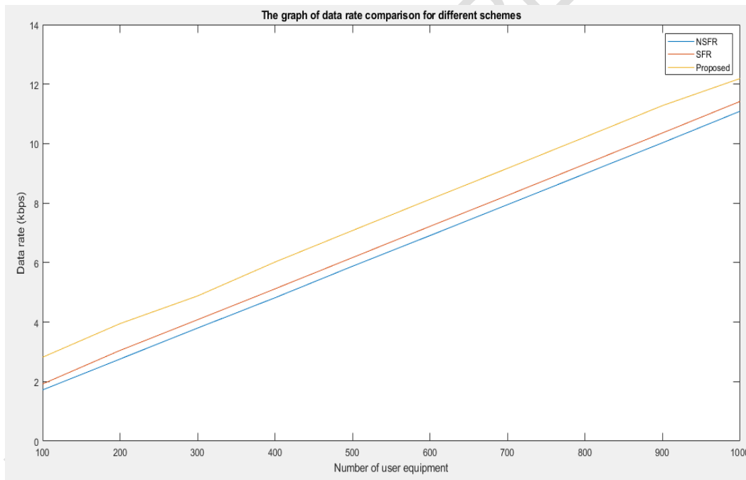
Figure 10. Data rate comparison for various schemes
