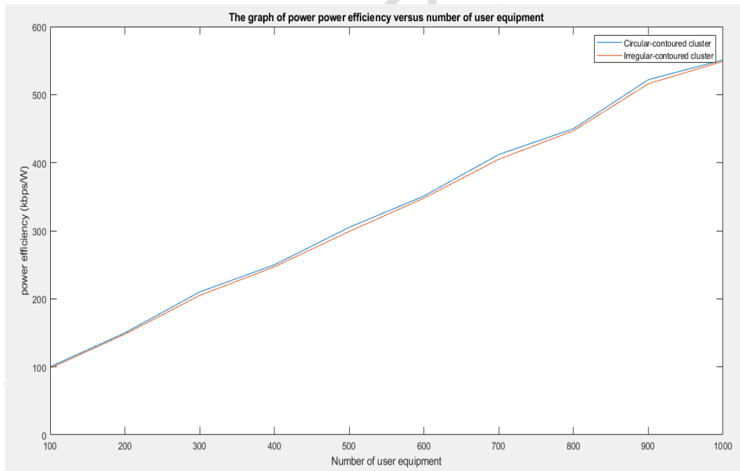
Figure 7. Power efficiency for circular-contoured cluster and irregular-contoured cluster
