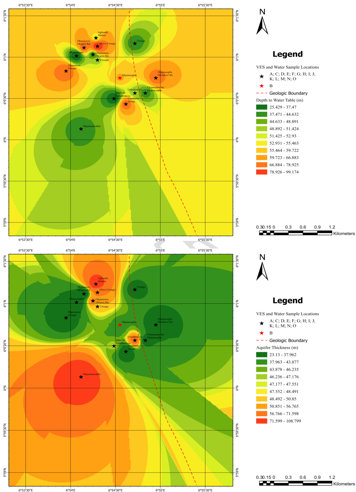
Fig.5: Spatial distribution of (a) water table and (b) aquifer thickness in the study area.
