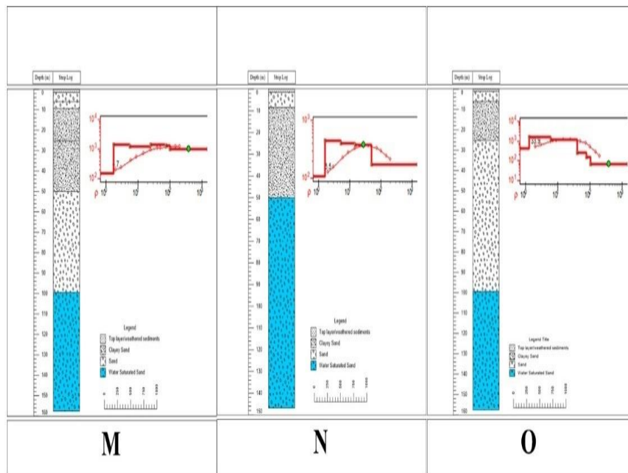
Fig.4: Strip Logs and corresponding VES curves A-O correspond to the different stations.
