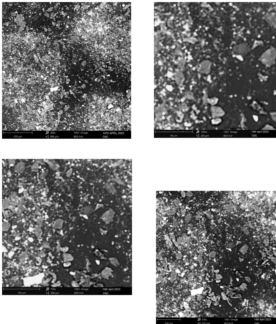
Fig. 2: SEM images of cellulose nanocrystals from alkali treated and bleached bean seed hulls
