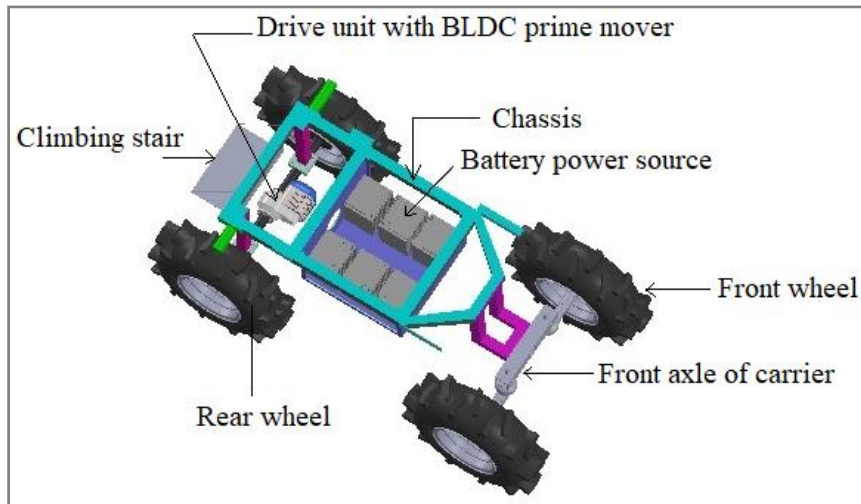
Fig. 1. Schematic sketch of aelectric multi-tool carrier power train
