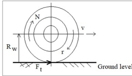
Fig. 3. Tractive effort developed by a driven wheel
