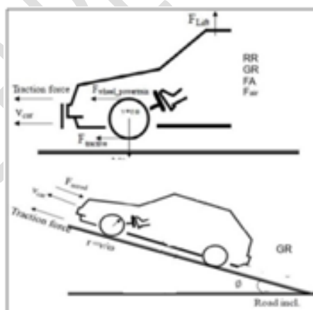
Fig.2. Forces acting on moving vehicle
