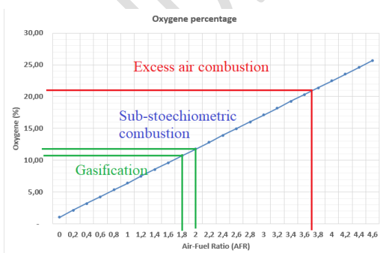
Figure 9 : Oxygene excess as function of AFR
