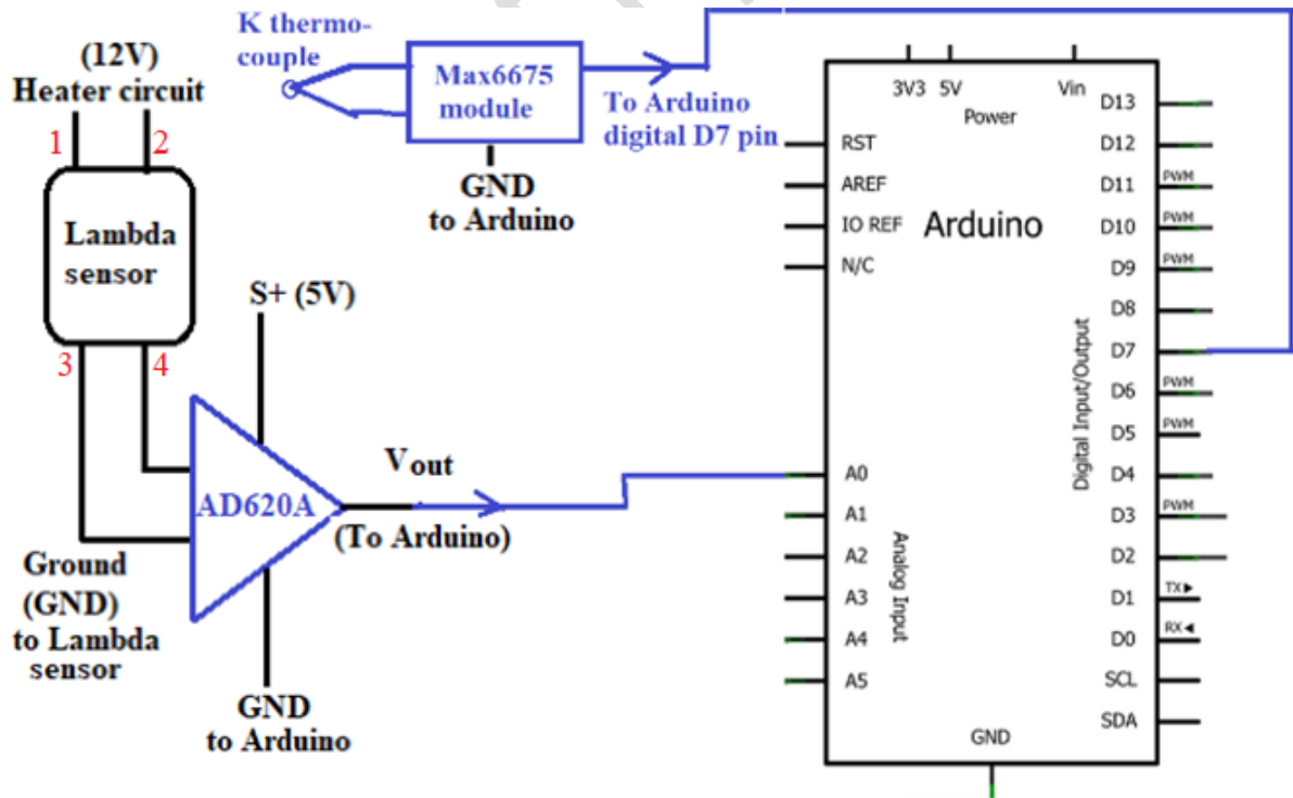
Figure 5: Electrical diagram of the monitoring system
