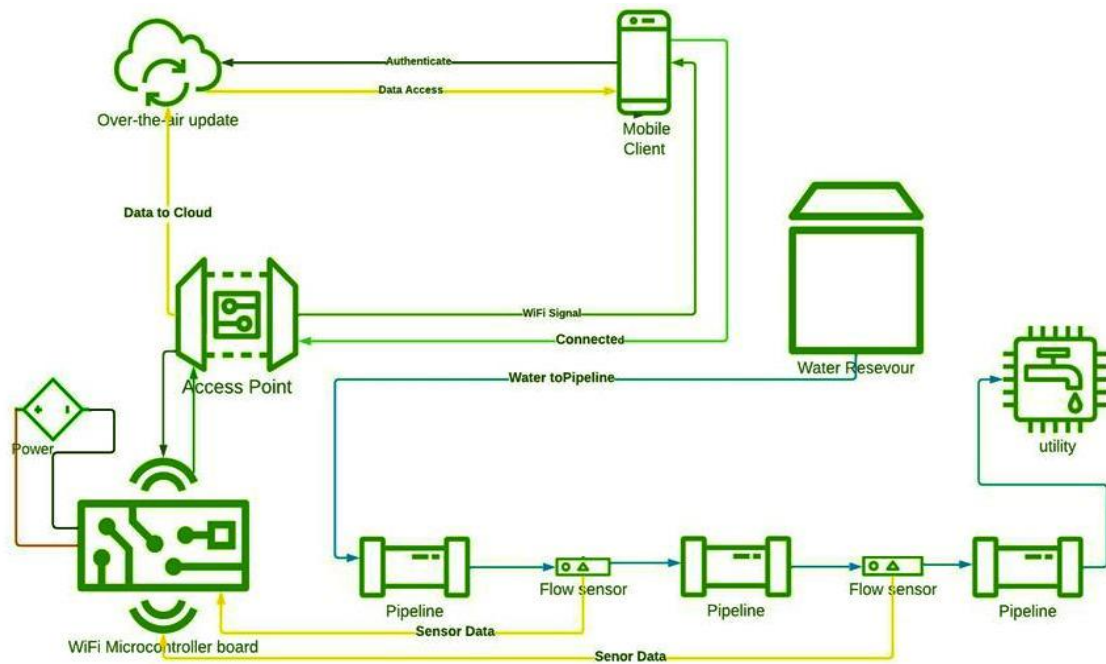
Figure 3: Water Leakage Detection and Localization Architecture
