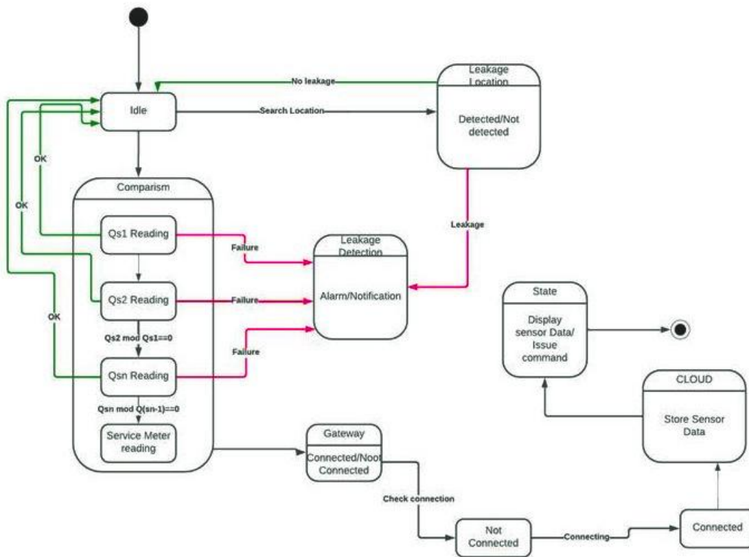
Figure 14: A Machine State Model for Leakage Detection
