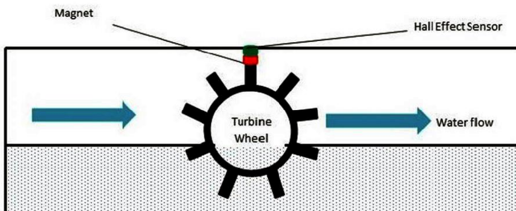
Figure 1: Pulse sampling and Counting
