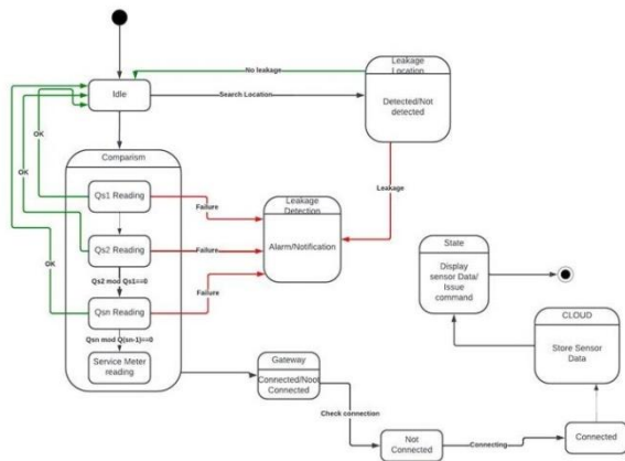
Figure 14: A Machine State Model for Leakage Detection
