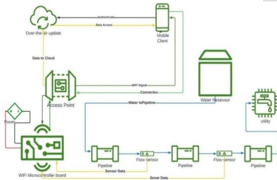
Figure 3: Water Leakage Detection and Localization Architecture
