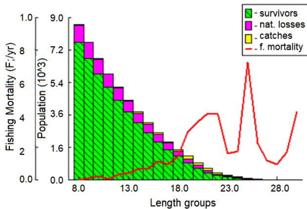
Fig. 8. Length-structured virtual population analysis of C. auratus
