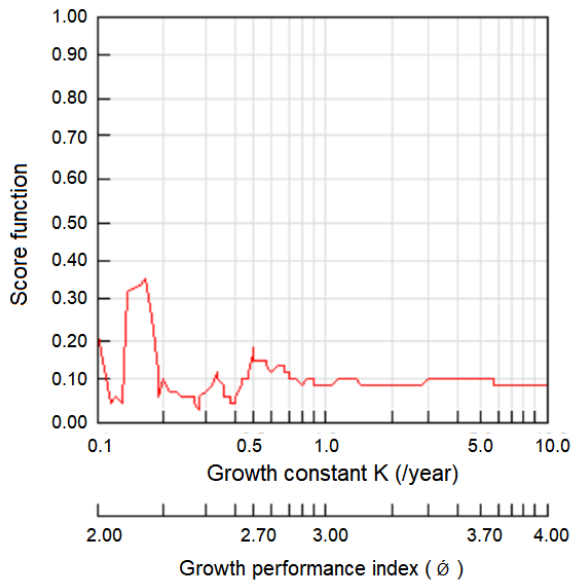
Fig. 2. K-scan routines of C. auratus
