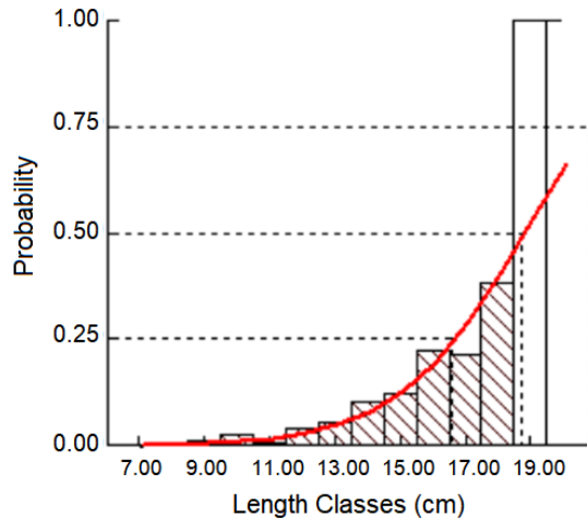
Fig. 5. Probability of capture for C. auratus
