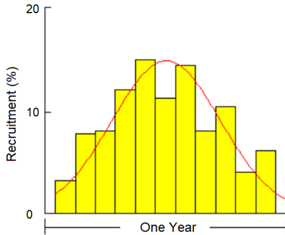
Fig. 6. Recruitment pattern of C. auratus
