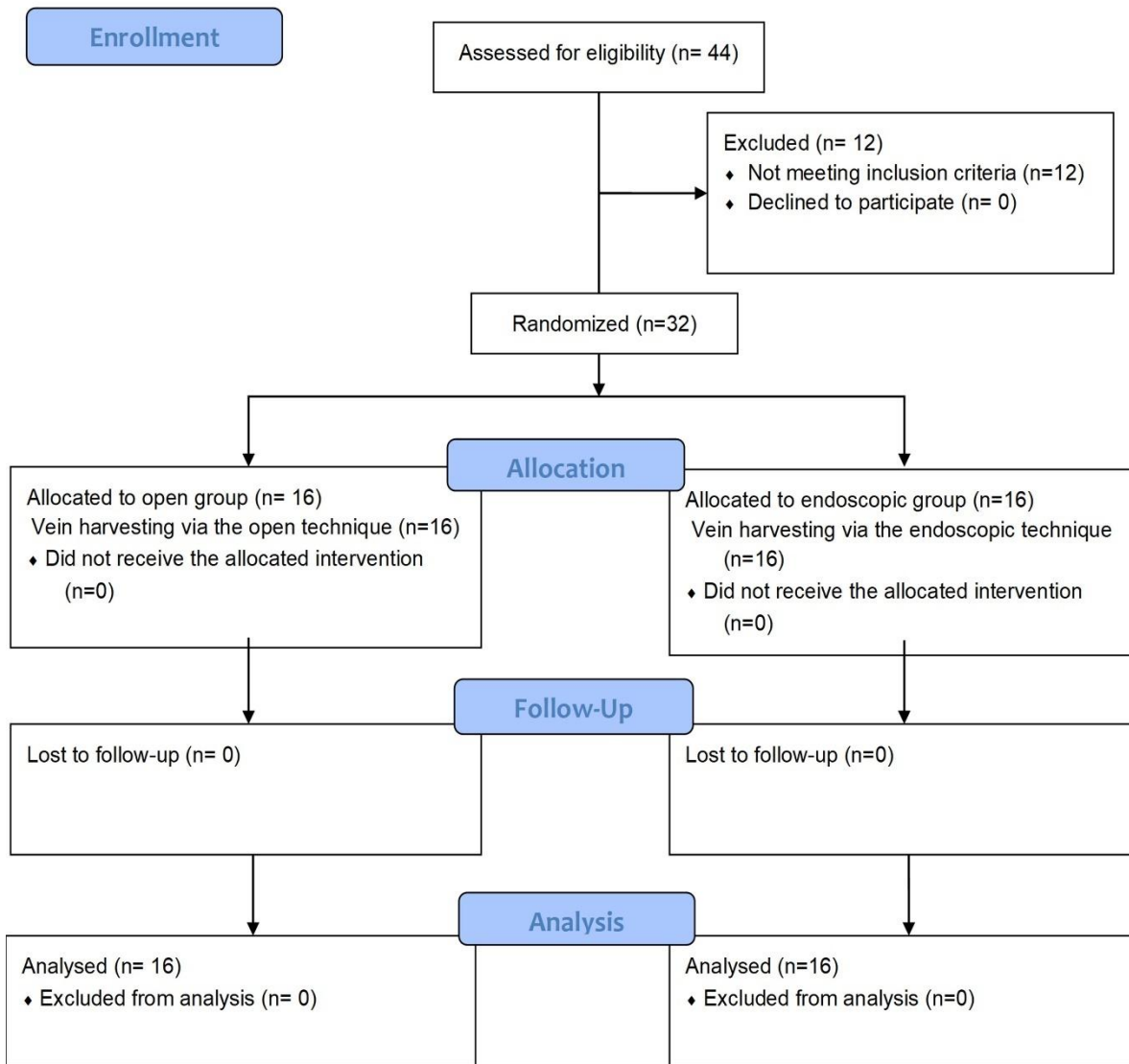
Figure 2: Consort flowchart of the studied patients
