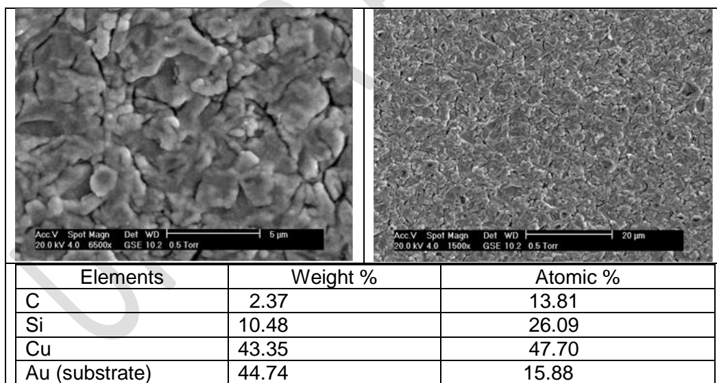
Figure 4 SEM micrograph of Cu electrodeposits with SiC nano particles from 0.1 M CuCl 2 , CTAB and 40 g / l SiC45-55nm in 1 ChCl: 2 EG based liquid at 0.8V and EDX map images shows of Cu, Si and C in the copper coating
