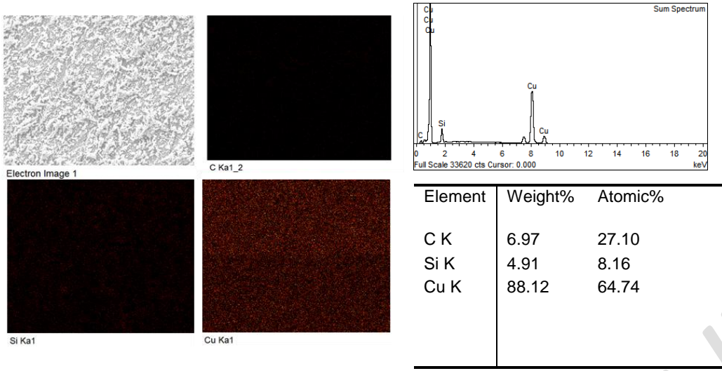
Figure 1 SEM microstructure of copper co-deposits film with silicon carbide 45-55 nm size
