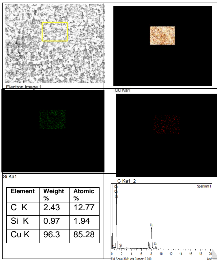
Figure 3 SEM micrograph of Cu electrodeposits with SiC nano particles from 0.1 M CuCl 2 , 1 mM SDS and 40 g / l SiC45-55nm in 1 ChCl: 2 EG based liquid at 0.8V and EDX map images show of Cu, Si and C in the copper coating.
