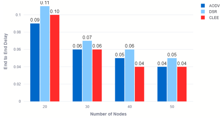
Figure 5: Delay against Number of sensor nodes
