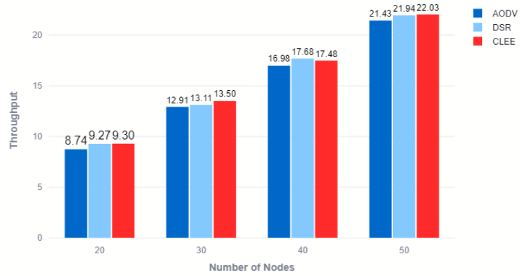
Figure 4: Throughput against Number of sensor nodes
