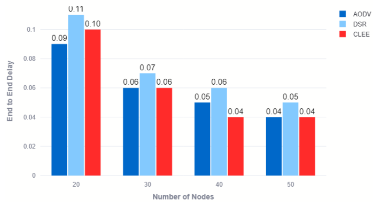
Figure 5: Delay against Number of sensor nodes
