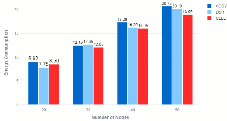
Figure 3: Energy Consumption against Number of sensor nodes
