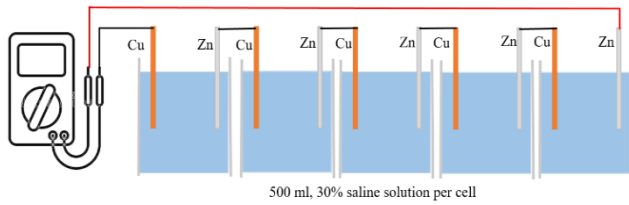
Figure 12 – Schematic diagram of parallel connection
