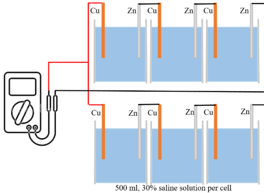
Figure 13 – Schematic diagram of series connection
