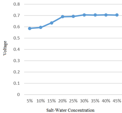
Figure 10 – Graph of voltage yield of Zinc-Copper electrode with different concentration.
