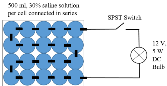
Figure 20 – Schematic diagram of a functional electrolytic cell with load
