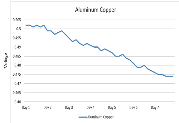
0.672 V is recorded on the last day of monitoring. Figure 9 – Decay Voltage of Aluminum-Copper
