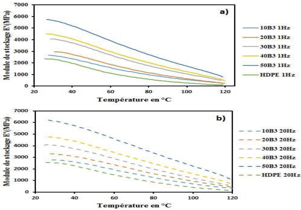
Fig. 1- Storage modulus E' with different wood fiber (birch) rates for frequencies a) 1Hz and b) 20Hz as a function of temperature
