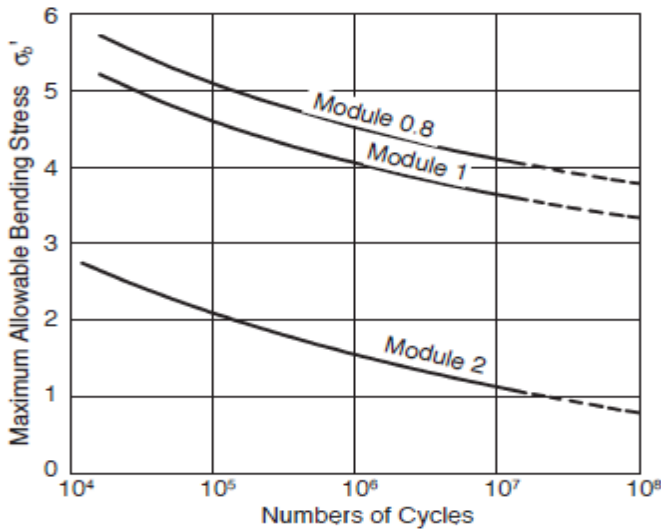
Fig. 2- Maximum allowable bending fatigue stress under ideal conditions for acetal M90.
