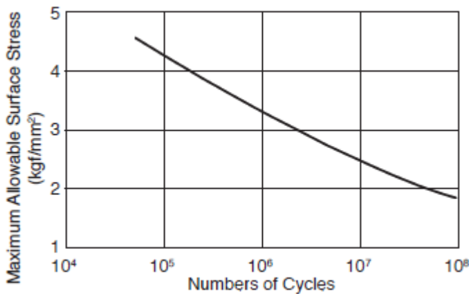
Fig. 5- Maximum allowable contact fatigue stress under the conditions specify here below for acetal M90:
