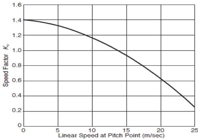
Fig. 3- Speed factor K_v for acetal M90
