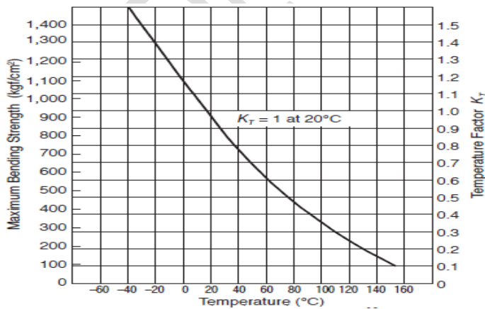
Fig. 4- Temperature factor K_T for acetal M90.
