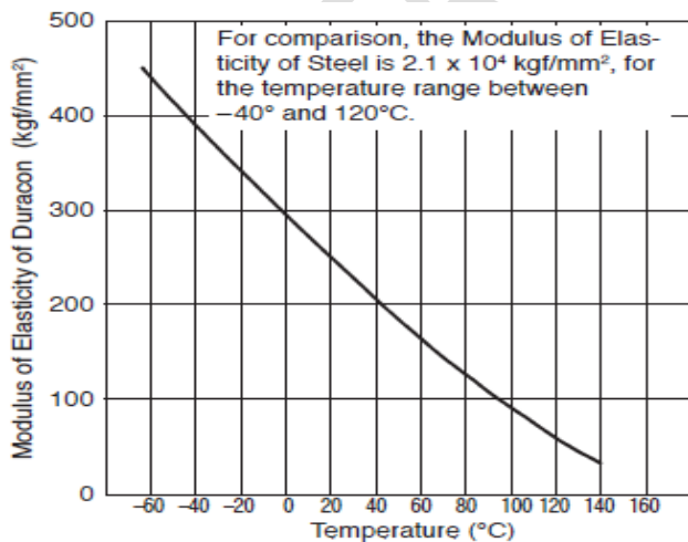
Fig. 6- Elasticity modulus as function of temperature for acetal M90
