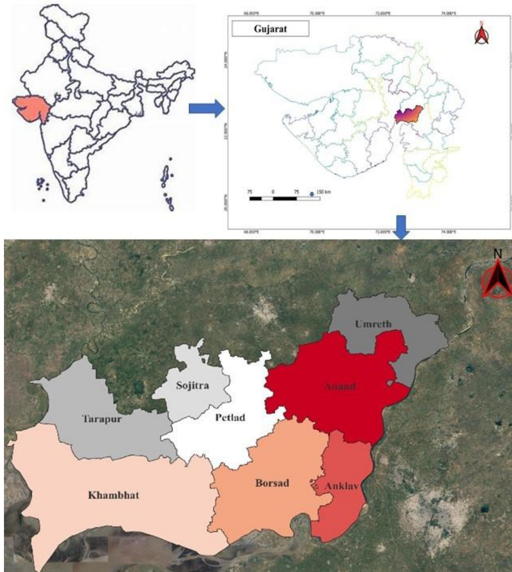
Figure 1. Test site location - Anand District of India
