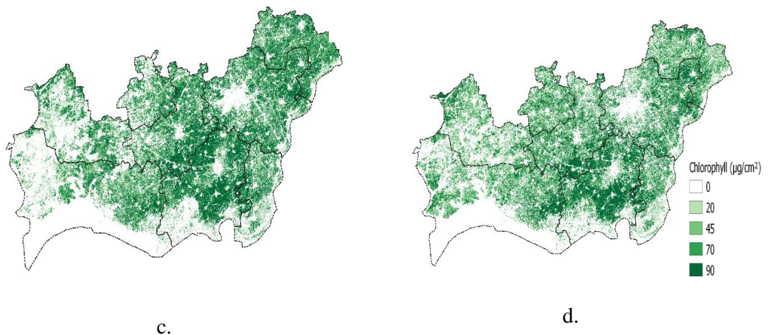
Figure 4: Chlorophyll retrieved for a. January, 2020 b. February 2020c. January, 2020 d. February 2020
