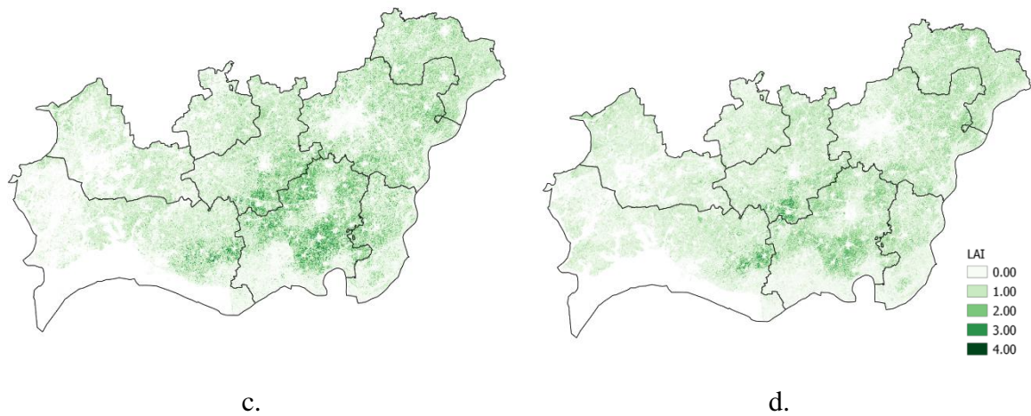
Figure 3: LAI retrieved (a) January 2020 (b) February 2020 (c) January 2021 (d) February 2021
