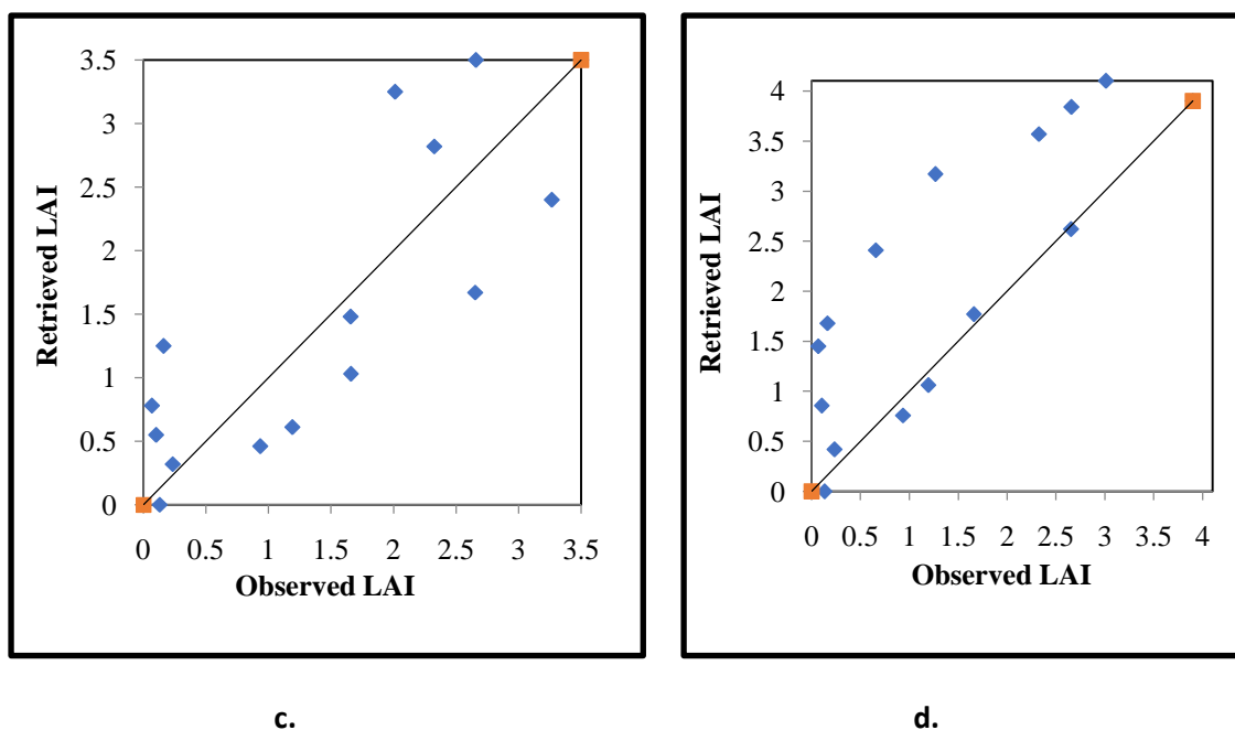
Figure 7: Retrieved versus measured LAI during rabi year 2020-21; a. Experimental plot, b. Navli research station field, c. Lambhvel tower field, d. Livestock research station field.
