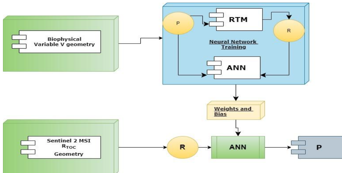
Figure 2: Flowchart for the retrieval of satellite-based biophysical parameters using SL2B algorithm in SNAP
