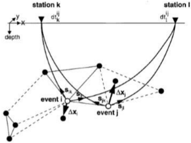
Figure 1. Illustration of the Double-Difference method [9]
