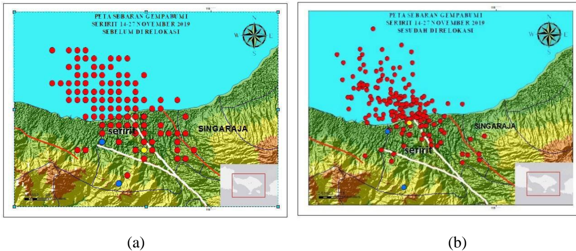
Figure 6. Earthquake distribution map (a) before relocation, (b) after relocation
