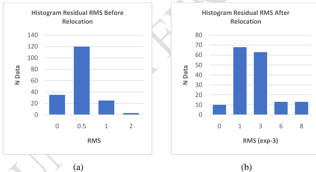
Figure 2. Histogram of RMS residual time values, (a) before relocation, (b) after relocation
