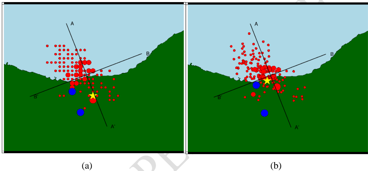
Figure 3. Results of cross section analysis of areas A-A' and B-B' (a) before relocation (b) after relocation
