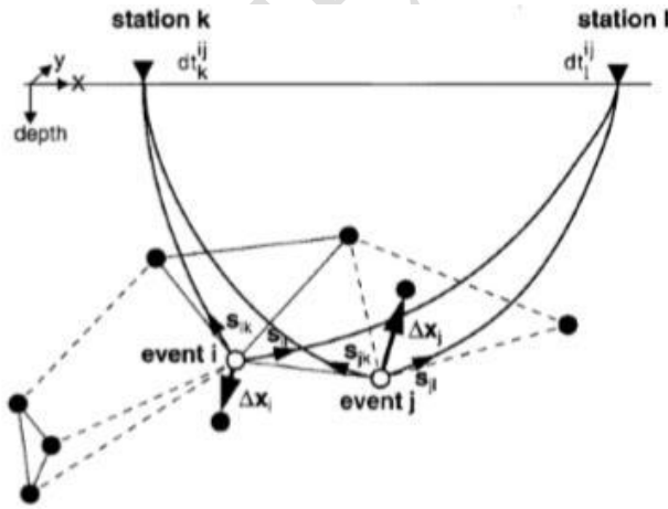
Figure 1. Illustration of the Double-Difference method [7]
