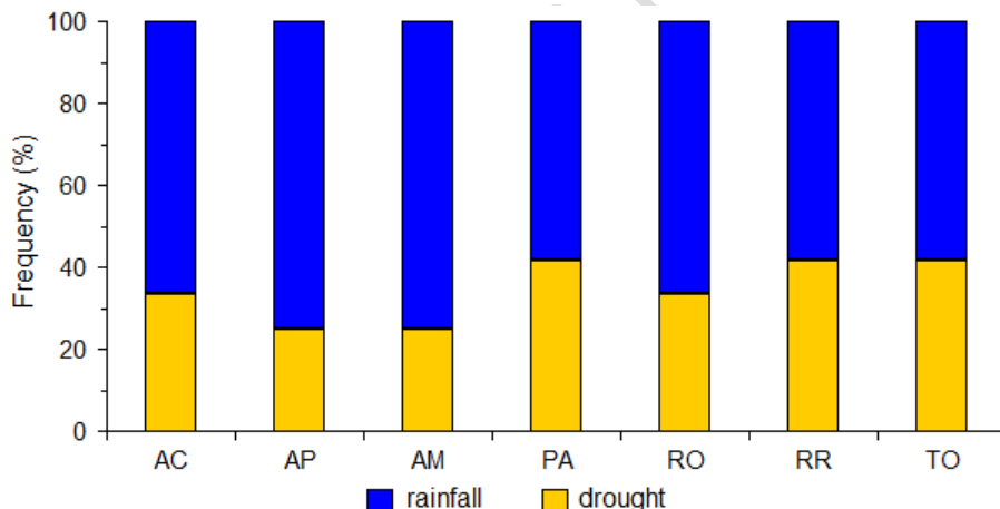
Figure 3: Annual frequency of rainfall and drought for the states of the North Region for the period from 1991 to 2022.
