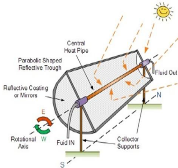
Fig.1. Parabolic Trough Collector [7]
