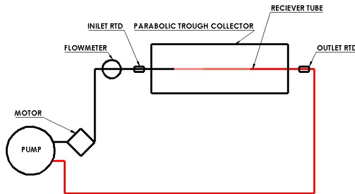
Fig.2 Schematic flow diagram of experimental set up.
