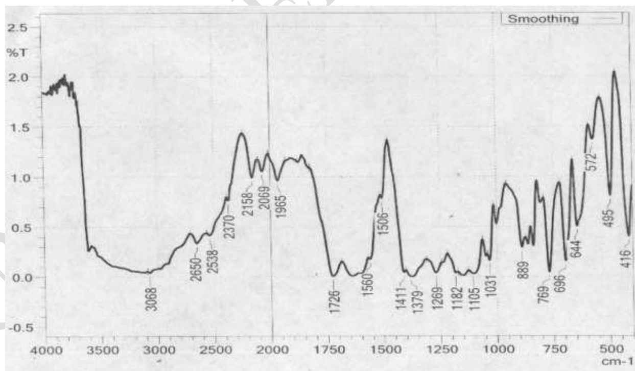
FT-IR spectrum of [Cu(INA) 2 ]-TH
