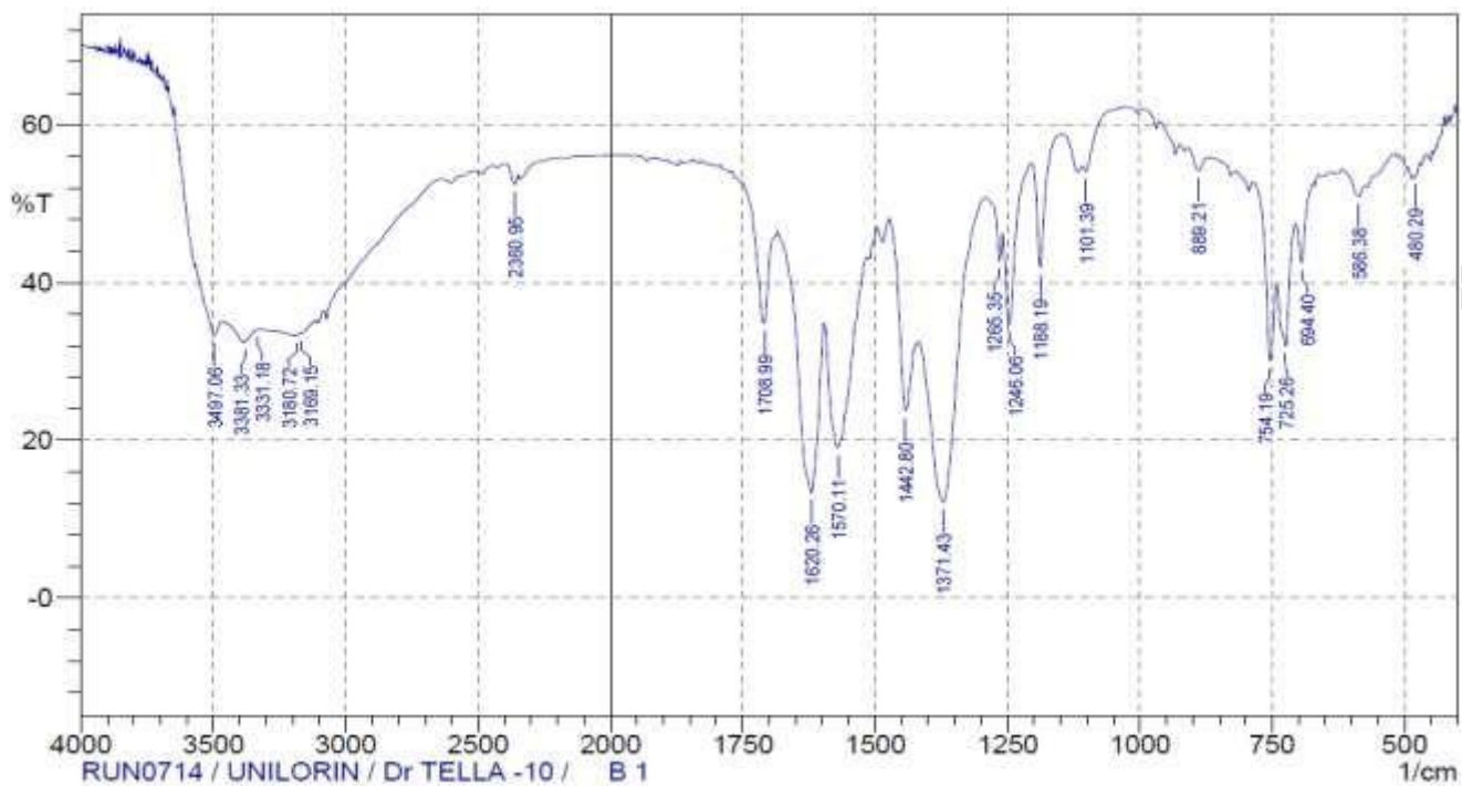
FT-IR spectrum of [\text{Cu}_3(\text{BTC})_2]
