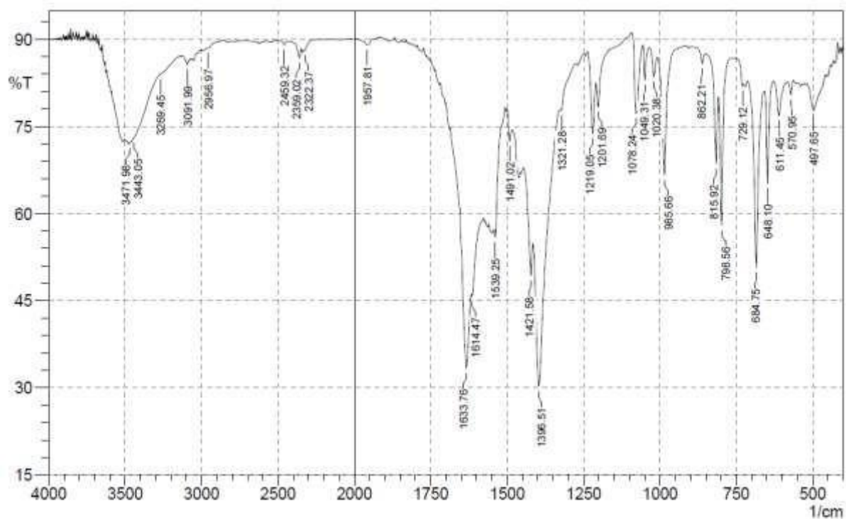
FT-IR spectrum of [Zn_2(Fum)_2(bpy)]
