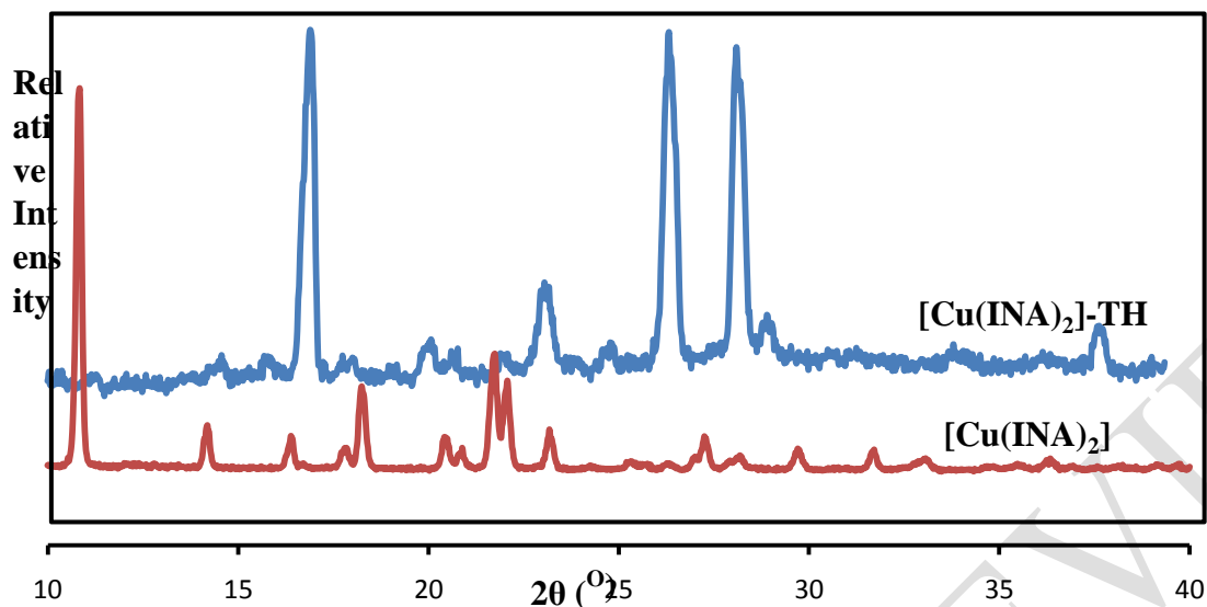
Fig. 6: XRPD pattern of [Cu(INA)_2] and thiol-modified [Cu(INA)_2]
