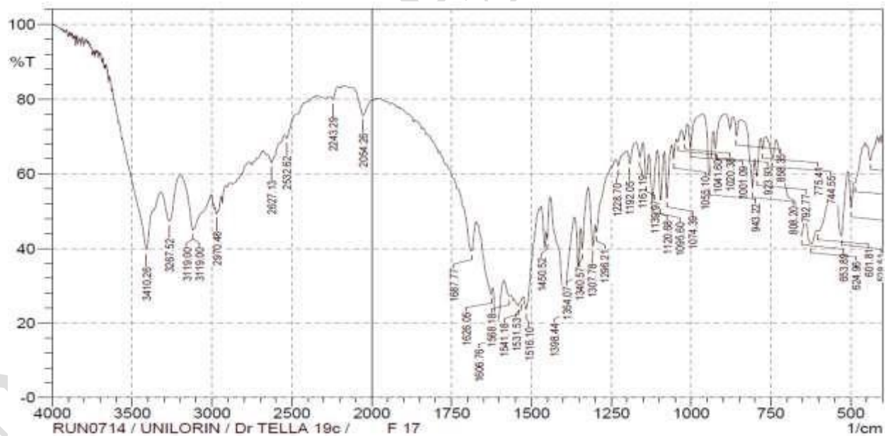
FT-IR of Glutaric acid
