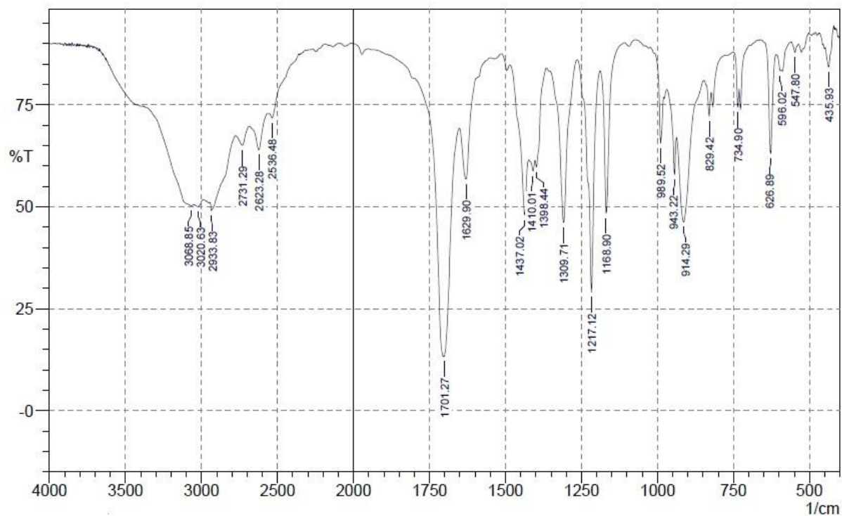
FT-IR spectrum of Itaconic acid
