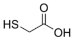
Figure 3: Structure of Thioglycolic Acid
