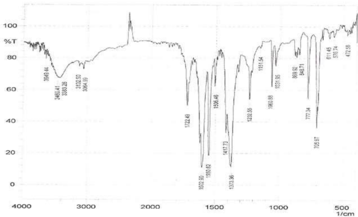
FT-IR spectrum of [\text{Cu}(\text{Ina})_2] \cdot \text{H}_2\text{O}
