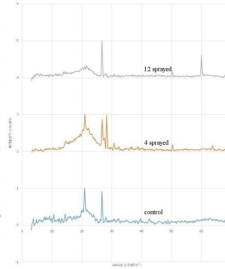
(c) PXRDS - Bitter gourd powder
