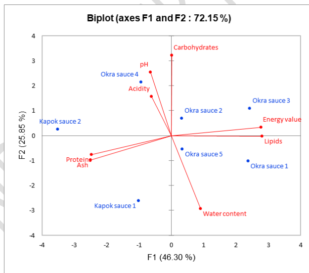
Figure 1. Result of principal component analysis of the physicochemical and nutritional characteristics of precooked sauces
